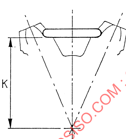
FIGURE 6 - Sprocket centre to bottom of pocket (Dimension K)
