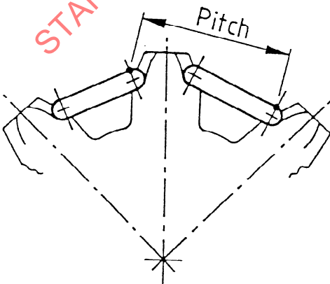
FIGURE 9 - Tooth pitch
