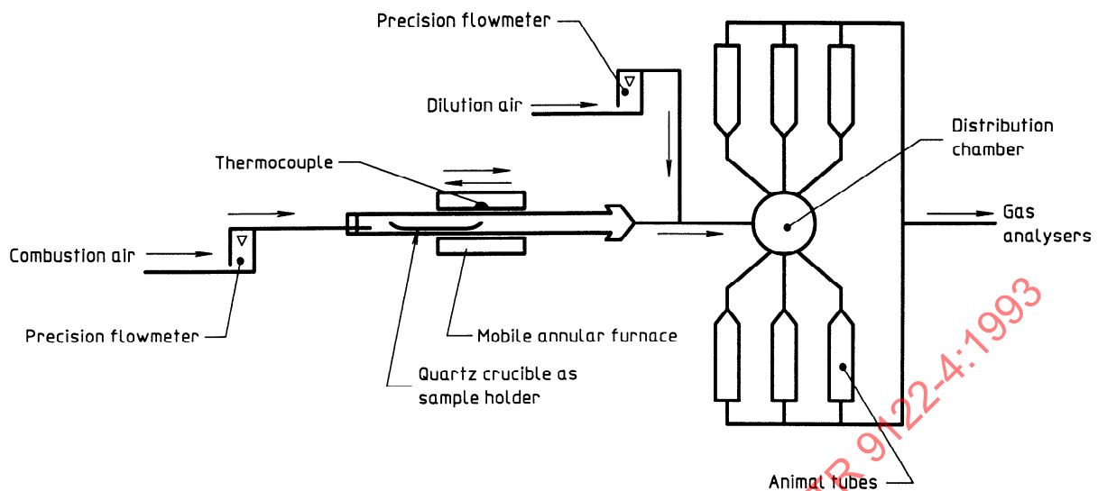
Figure 4 — DIN 53436 smoke toxicity apparatus including tube furnace
