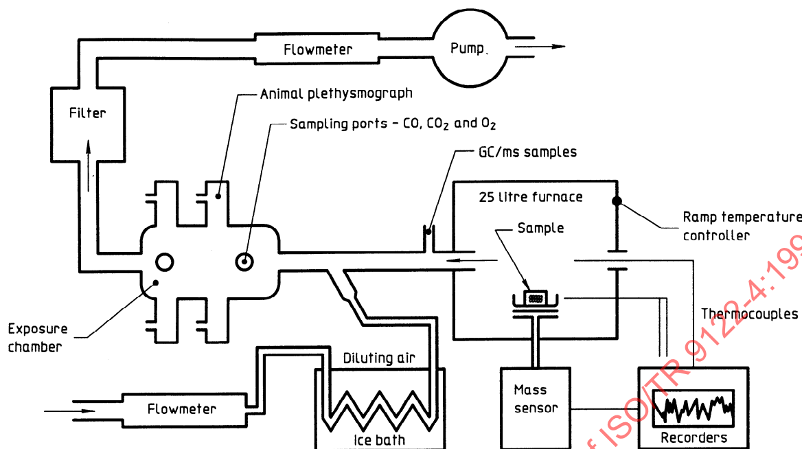
Figure 3 — UPitt smoke toxicity apparatus including box furnace
