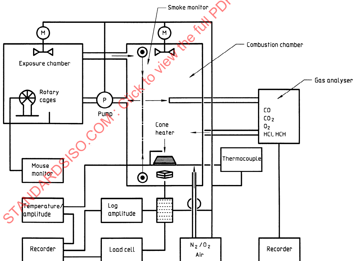
Figure 9 — RIPT smoke toxicity apparatus including cone furnace
