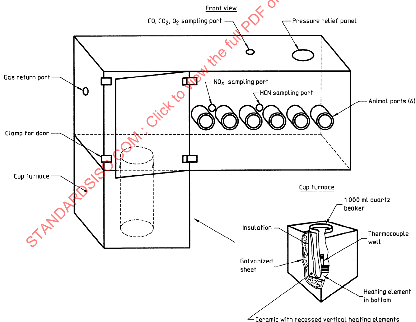
Figure 2 — NBS cup furnace smoke toxicity apparatus
