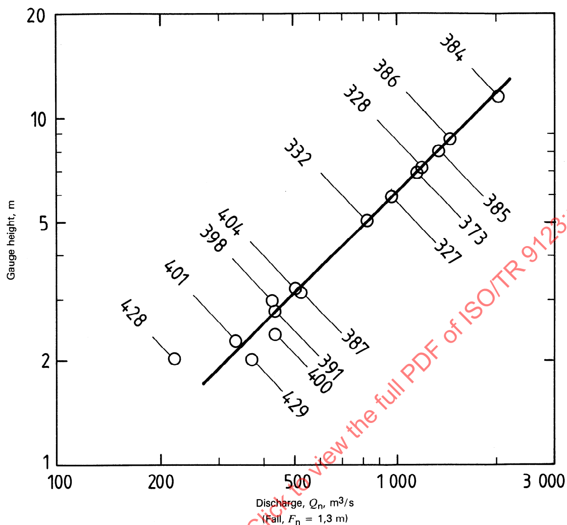
Figure 2 — Constant-fall rating
