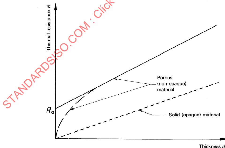
Figure 1 — Thermal resistance as a function of thickness for opaque and non-opaque materials
