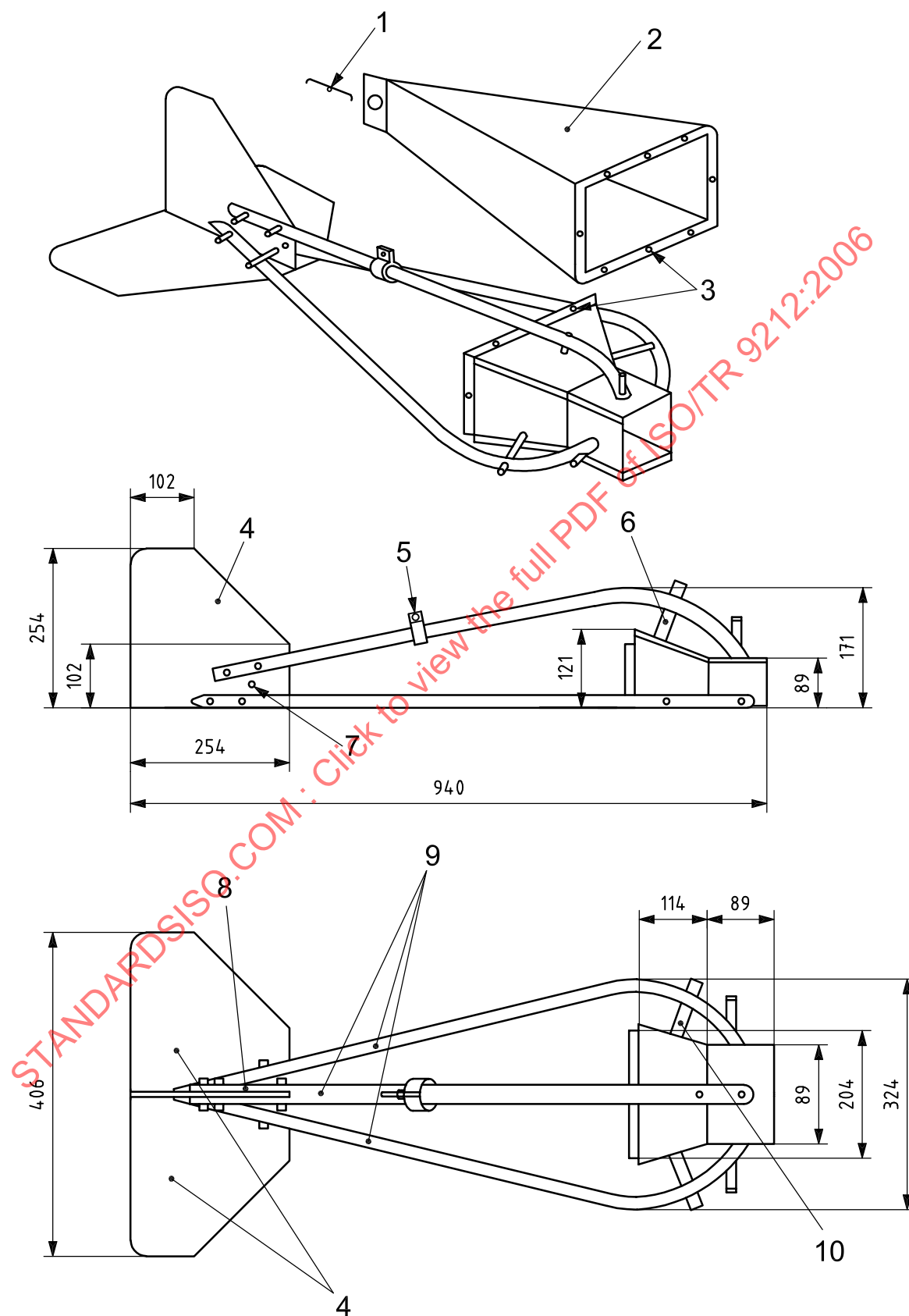
Figure 3 — Helley-Smith bedload sampler
