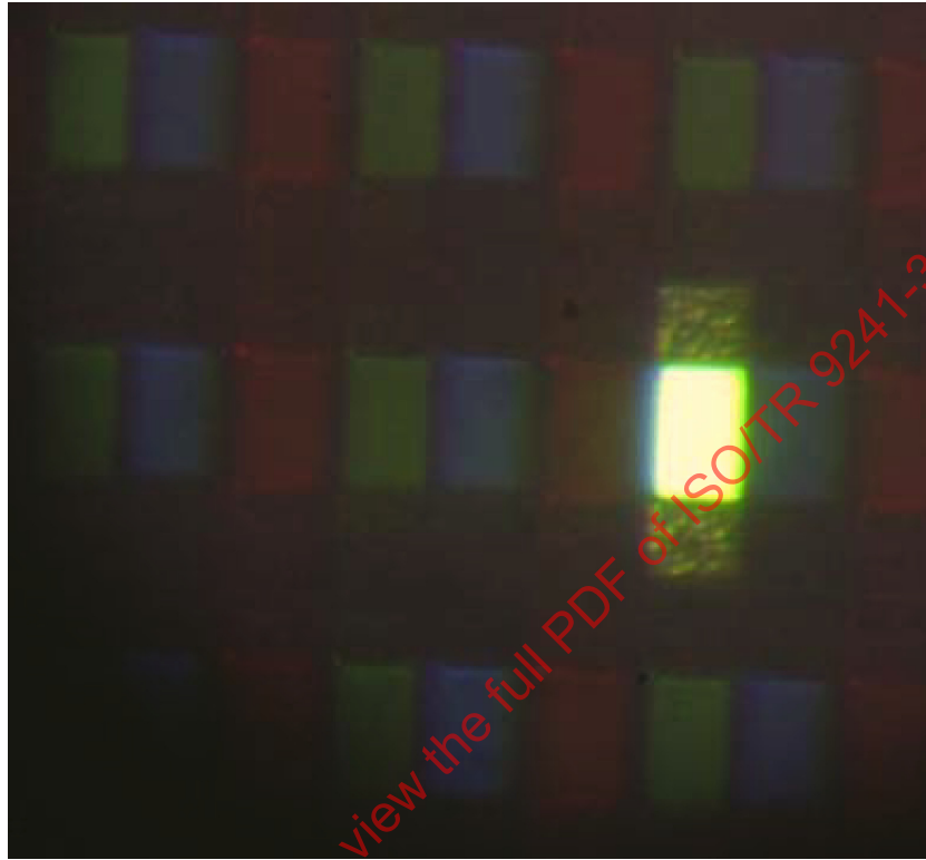
Figure 16 — Subpixel defect in a transfective LCD in dark
