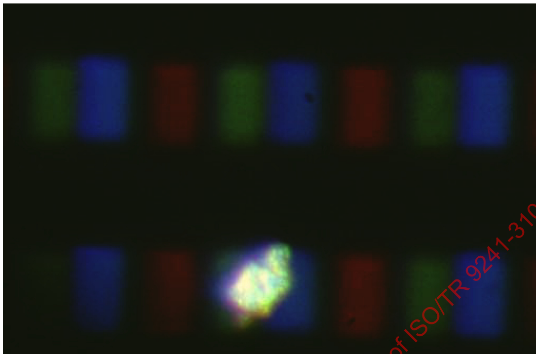
Figure 21 — Non-pixel-related defect in a transfective LCD
