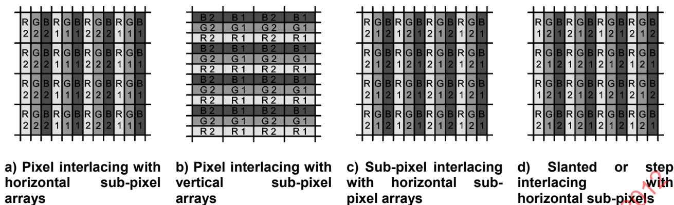
Figure 11 — Different pixel interlacing example illustrations assuming square (R,G,B) pixels in two-view displays
