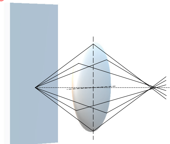
Figure 35 — Astigmatism
