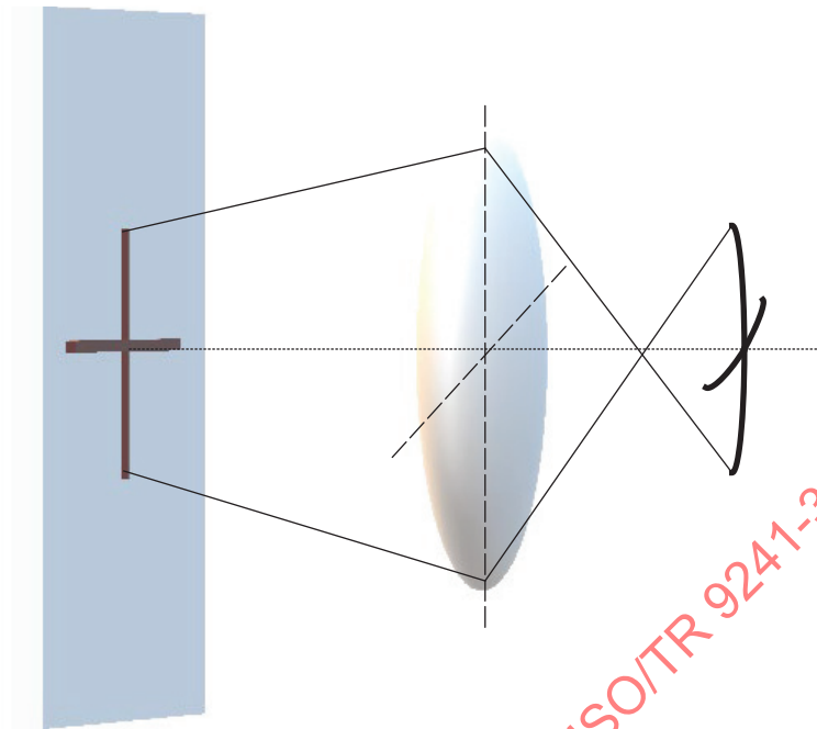
Figure 36 — Curvature of field
