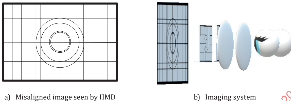
Figure 44 — Enlargement misalignment
