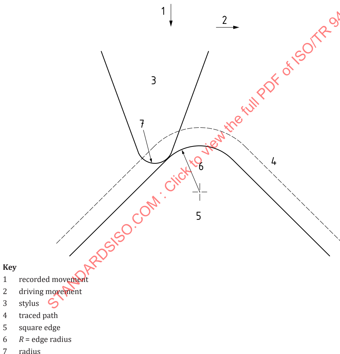
Figure 2 — Paper-recording roughness method
