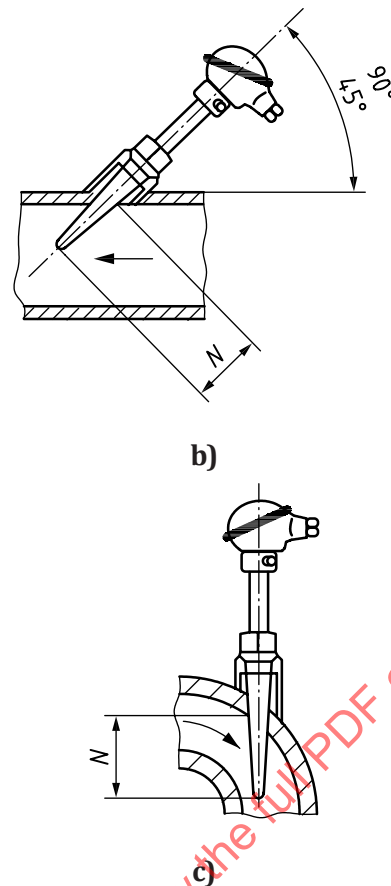
Figure 12 — Installation of immersion temperature probe
