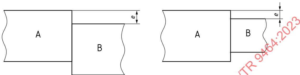
Figure 7 — Inspection of measuring pipe sections
