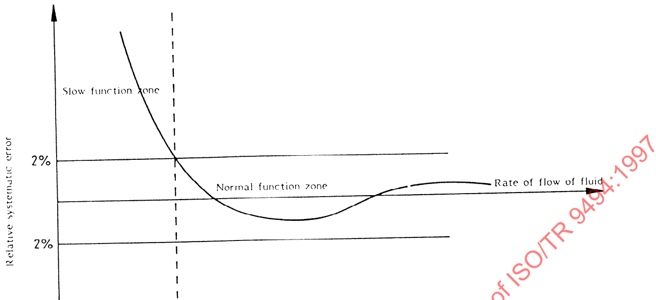
Figure 4 - Relative systematic error function for a flowmeter
