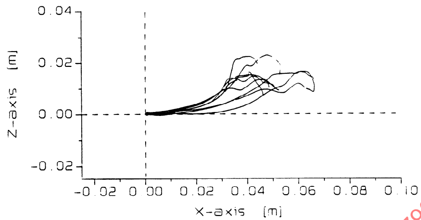
Fig. 3 T1 origin trajectories with respect to sled
