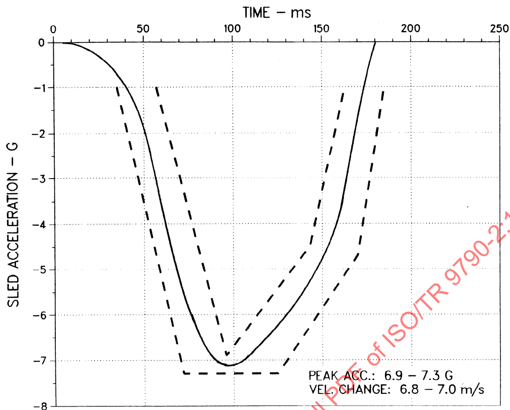
FIGURE 6. SLED PULSE ENVELOPE
