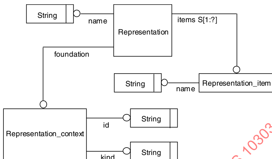
Figure C.1 - ARM EXPRESS-G diagram 1 of 1
