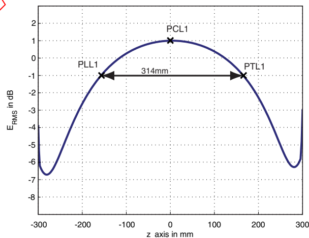
Figure M.1 – E_z -field induced in the ASTM phantom along line L1 (0 dB = 71V/ \mu T)
