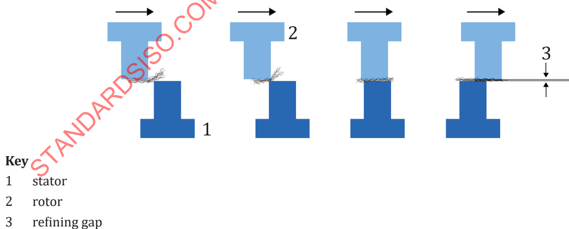
Figure 1 — Bar-to-bar refining principle
