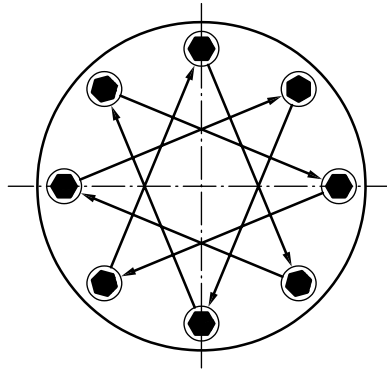
Figure 4 — The sequence of tightening the bolts
