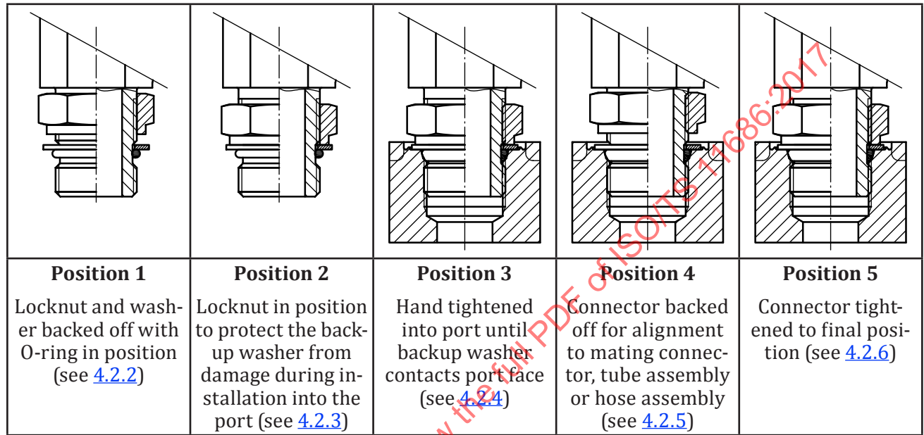
Figure 1 — Instructions for assembling connectors with adjustable stud ends and O-ring sealing
