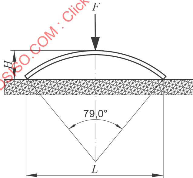
Figure A.5 — Principle of testing with the 79 ° segmental test piece
