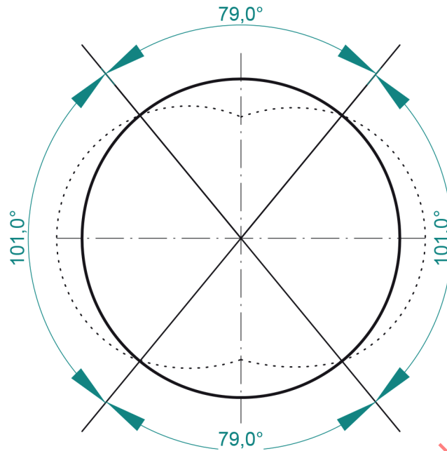
Figure A.4 — Locations of four test pieces
