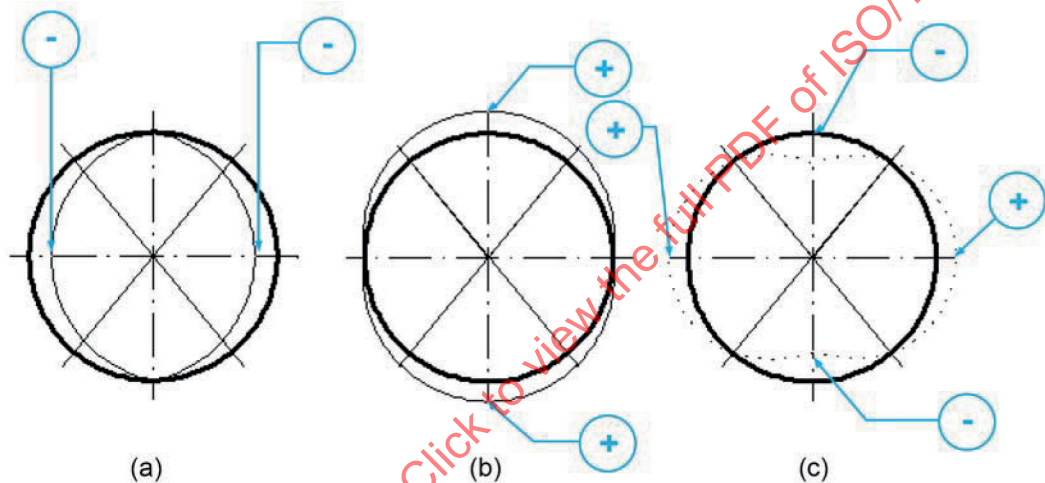
Figure A.2 — Distribution of a) normal force, b) transverse force, c) bending moment
