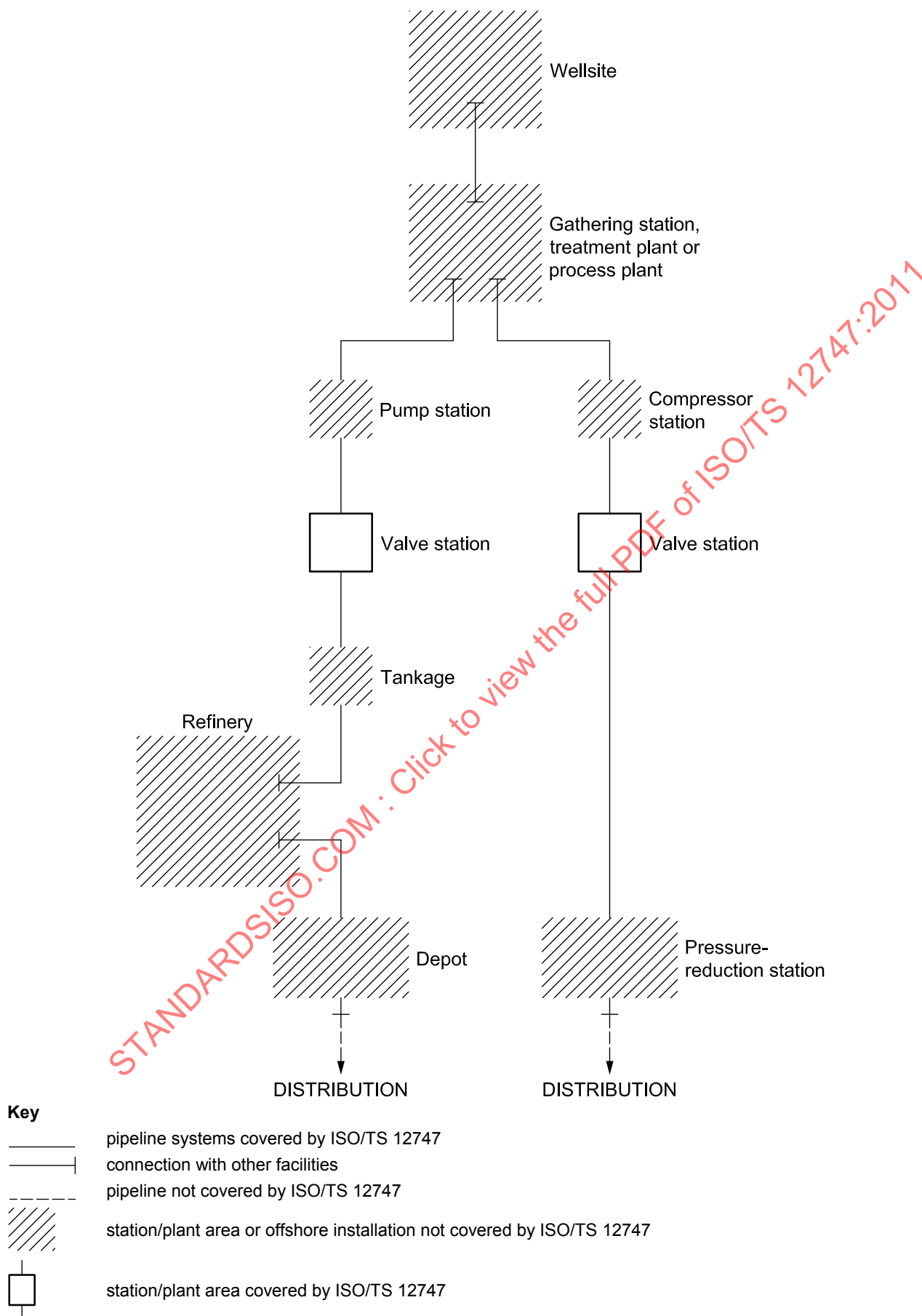
Figure 1 — Extent of pipeline systems covered by this Technical Specification
