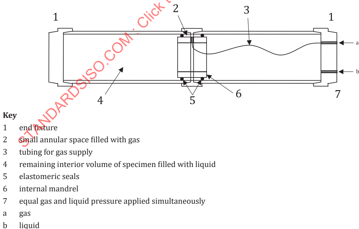
Figure 18 — Illustrative example set-up for limit-strain test
