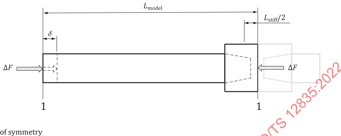
Figure A.3 — Schematic for calculation of high-stiffness interval
