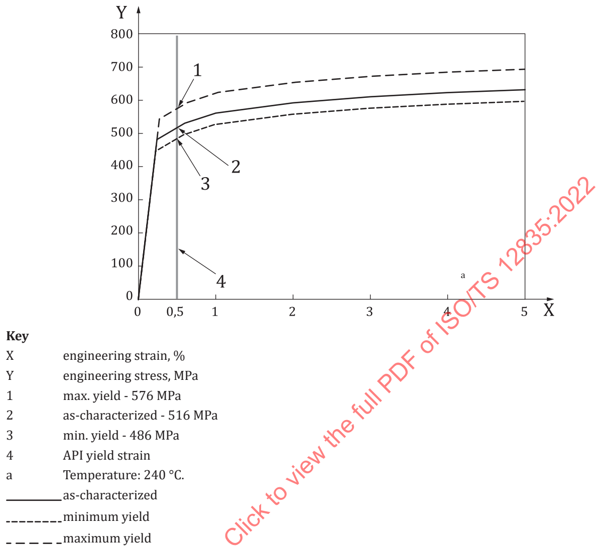
Figure 10 — Example of ASL-240 material properties
