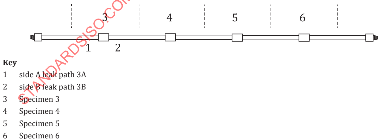
Figure 2 — Illustration of connection string assembly
