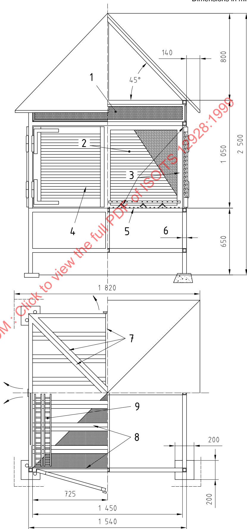
Figure C.1 — Outside shelter
