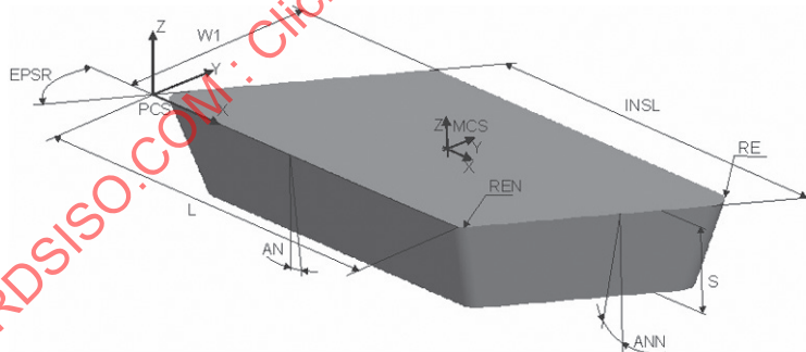
Figure 40 — Parallelogram non-equilateral shaped insert with corner radius
