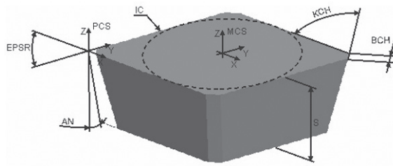
Figure 13 — Square insert with corner chamfer
