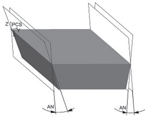
Figure 36 — Parallelogram non-equilateral shaped insert with trim planes for major clearance angles
