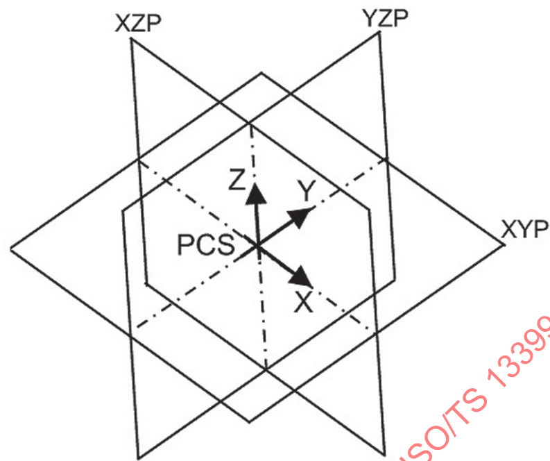
Figure 1 — Reference coordinate system “PCS”
