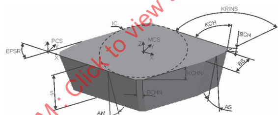
Figure 16 — Rhombic insert with wiper edge and corner chamfer
