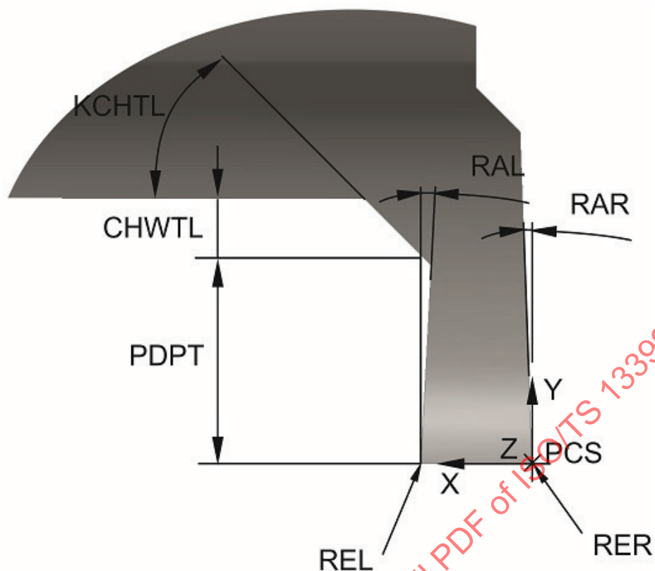
Figure 16 — Determination of properties for cutting profile
