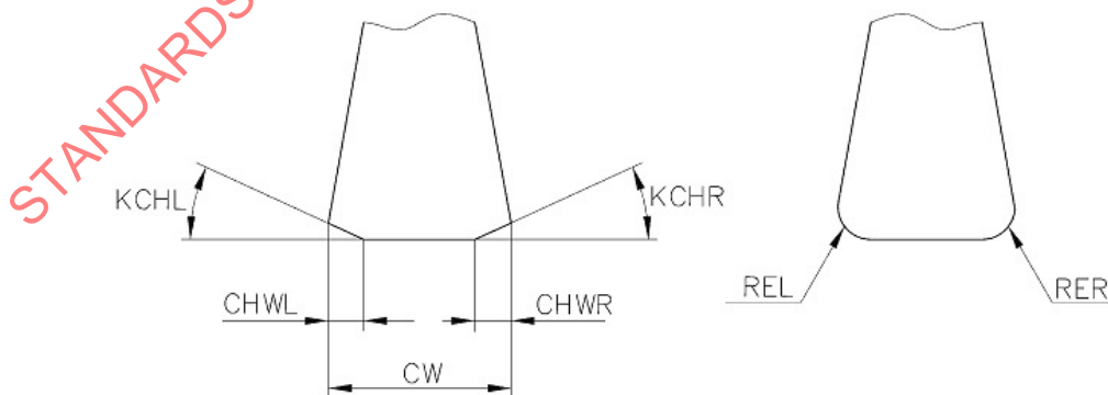
Figure 8 — Corner chamfer width, corner chamfer angle, corner radius
