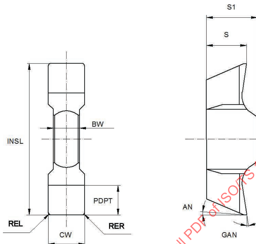
Figure 19 — Determination of properties for a self-clamping grooving insert with two cutting edges
