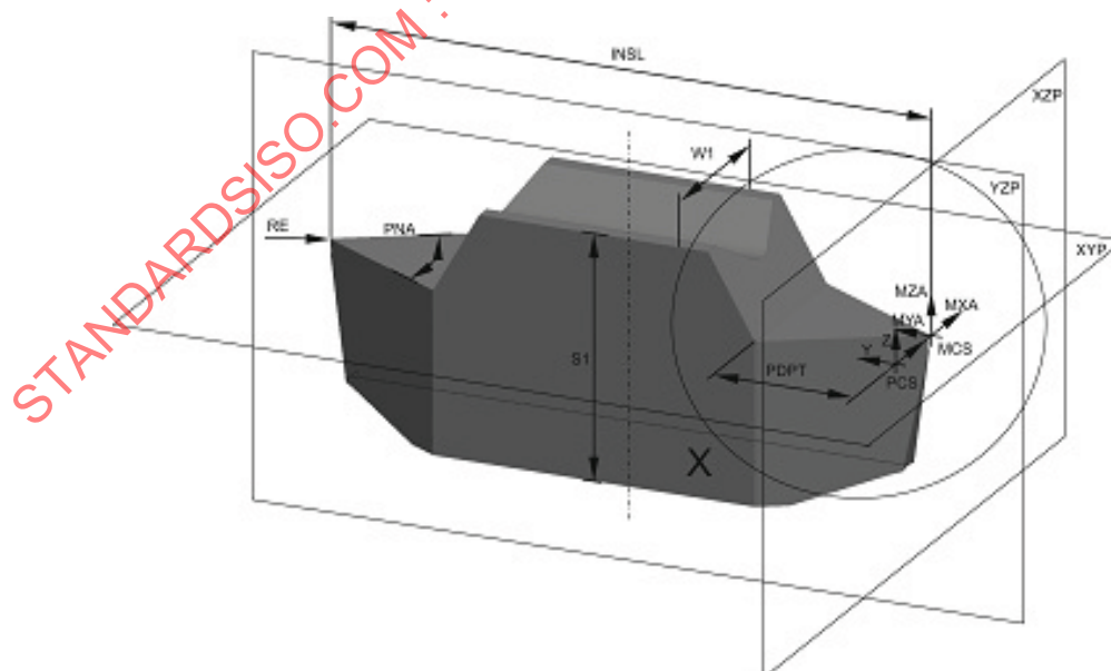
Figure 26 — Profiling and partial threading insert with two cutting edges: basic model
