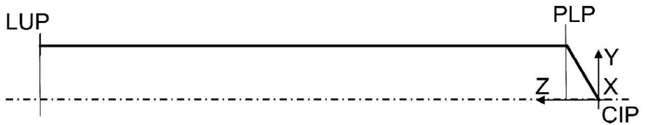
Figure 8 — Twist drill — Sketch of the cutting part
