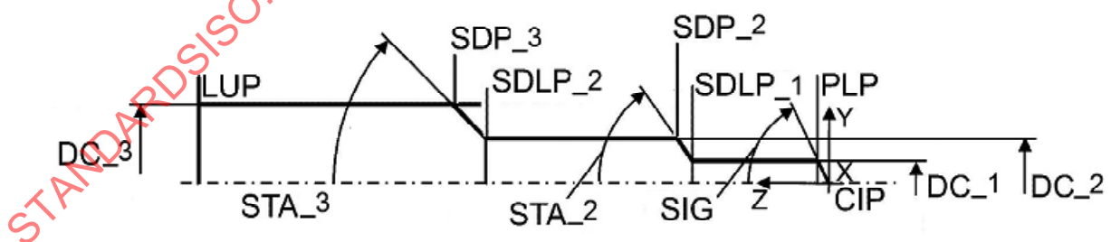
Figure 12 — Step drill — Sketch of cutting part
