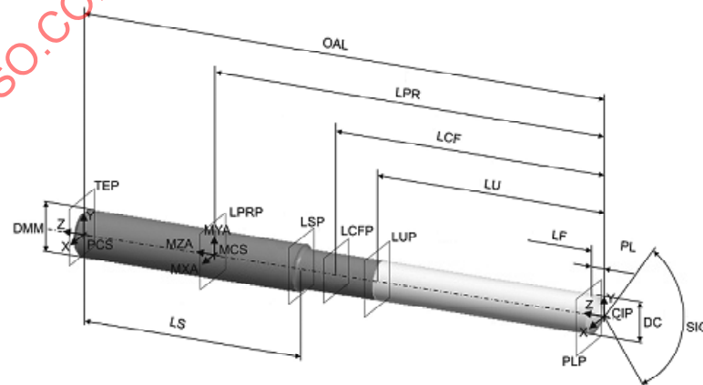
Figure 10 — Twist drill — Complete
