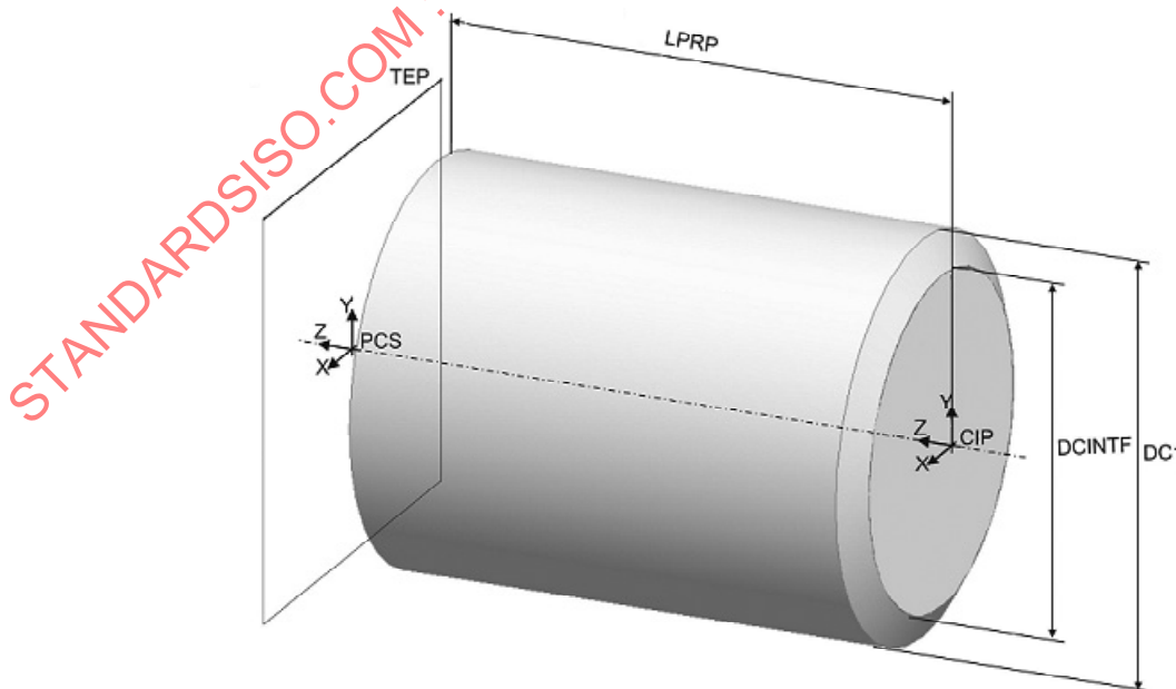
Figure 46 — Shell core drill — Revolved body of cutting part
