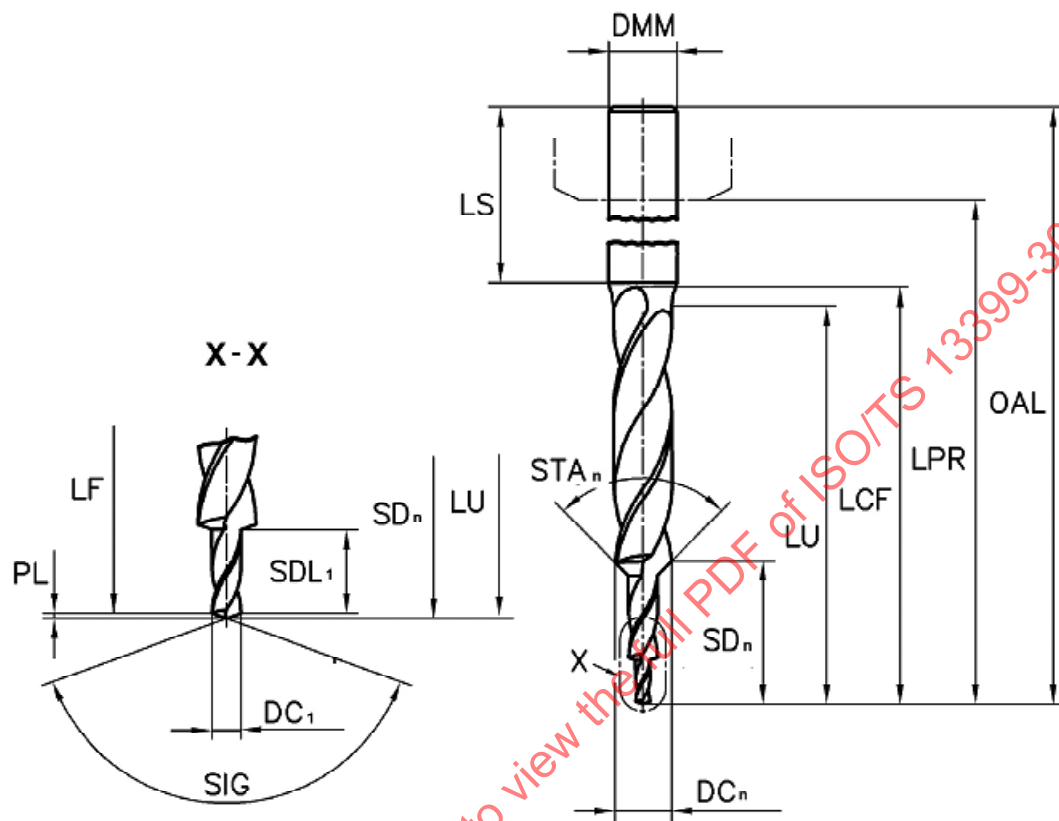
Figure 11 — Step drill — Determination of properties
