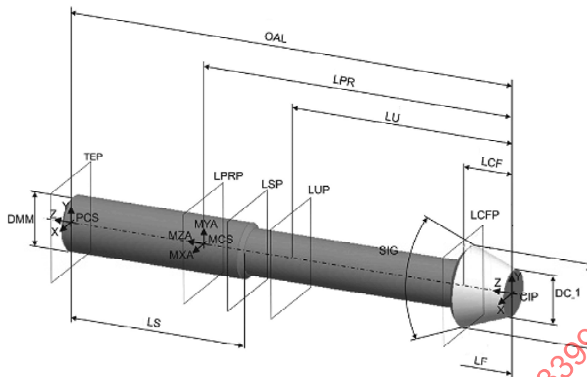
Figure 30 — Tapered countersinking tool — Complete
