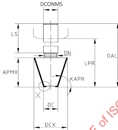
Figure 17 — V-groove end mill; Determination of properties
