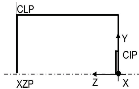
Figure 44 — Thread end mill: Sketch of cutting part
