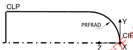
Figure 32 — Ball-nosed end mill: Sketch of cutting part
