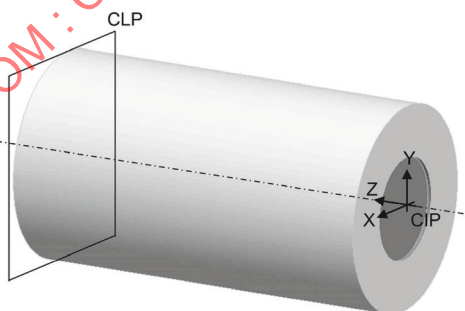
Figure 11 — Non-centre cutting end mill: Revolved body of cutting part
