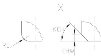
Figure 7 — Detail X
