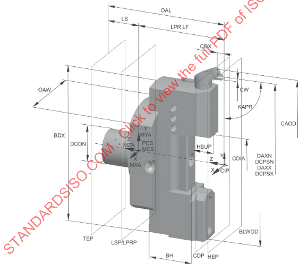
Figure 41 — Assembled single-point bridge tool for axial grooving
