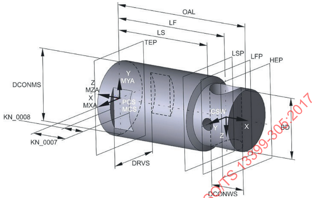
Figure 28 — 3D models of a boring head for adjustable units
