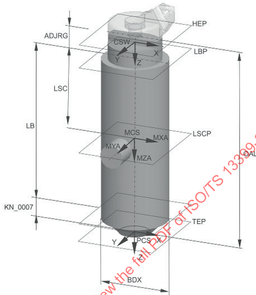
Figure 26 — 3D model of an adjustable unit
