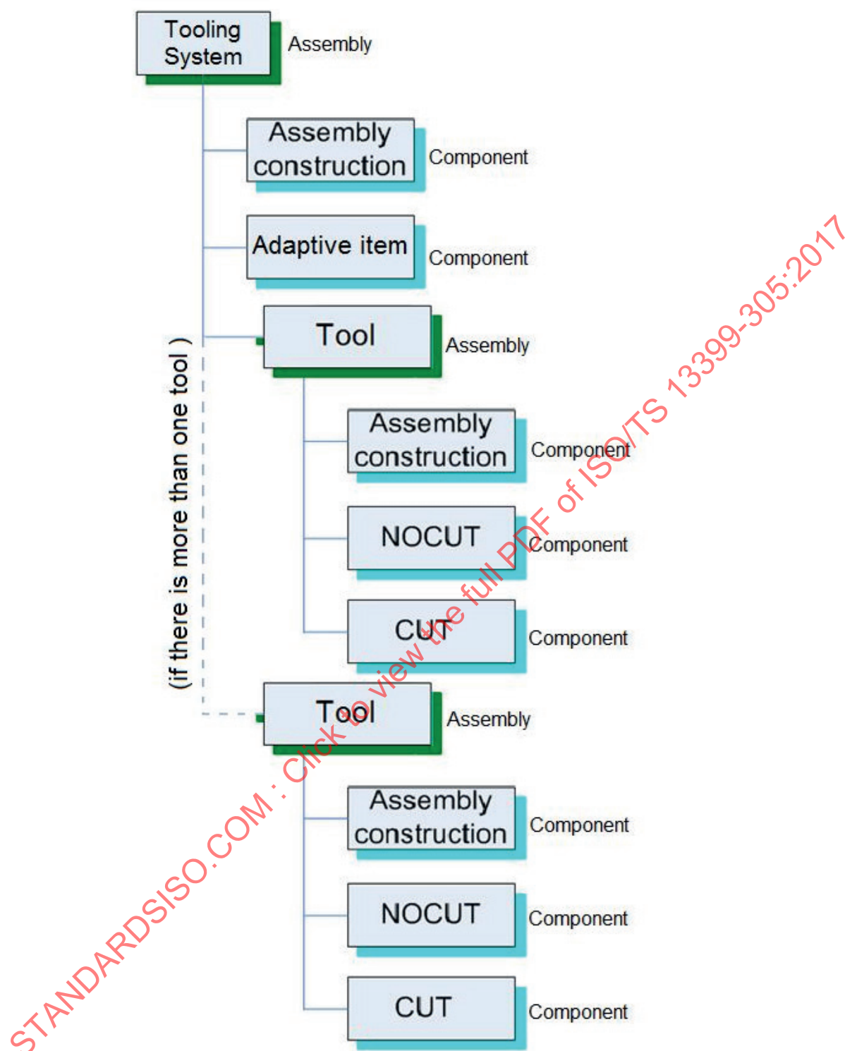
Figure 53 — Model for data exchange
