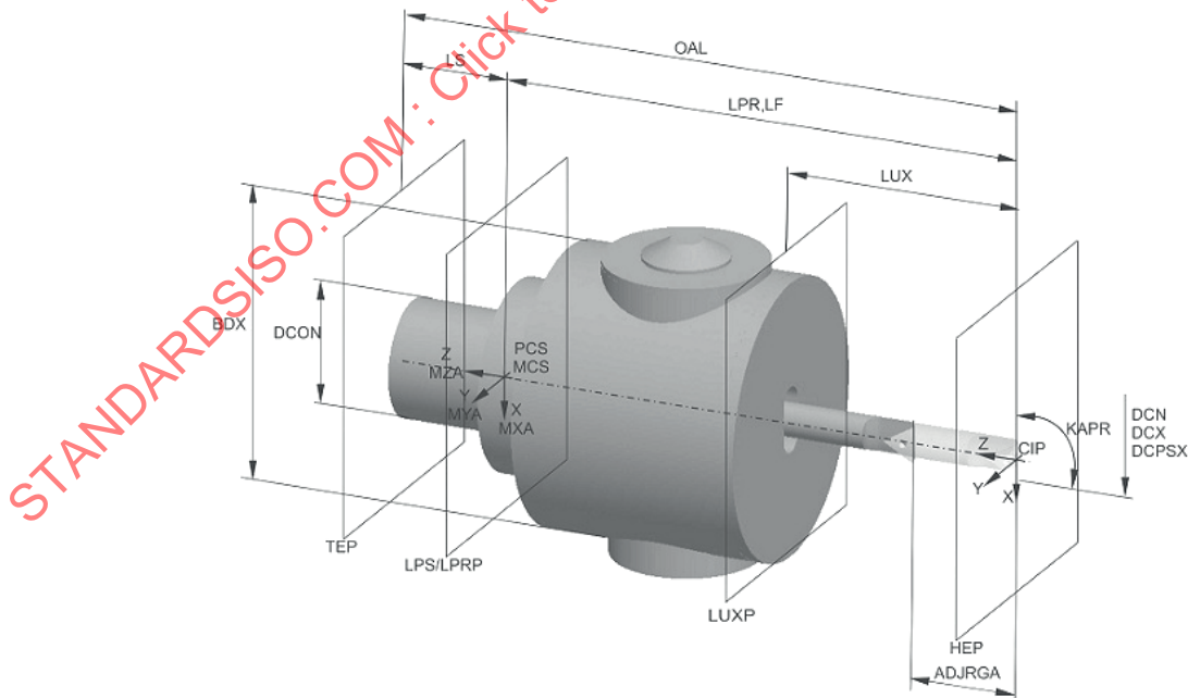
Figure 47 — Assembled fine boring head with boring bar
