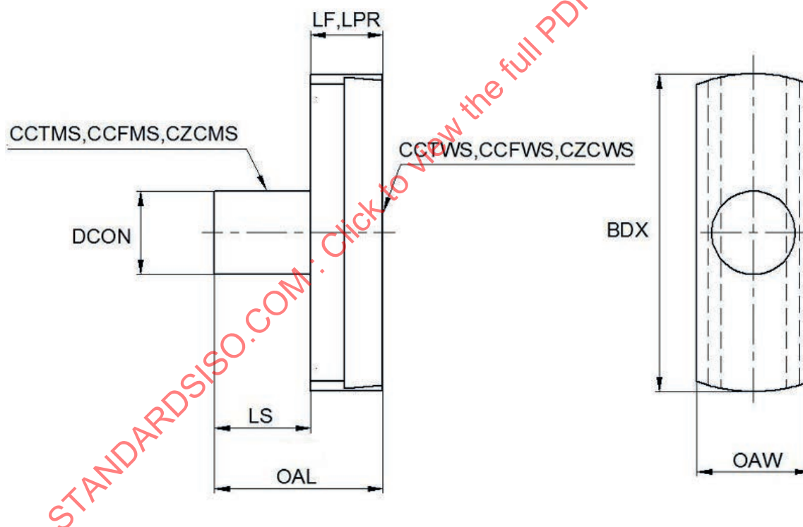
Figure 12 — Determination of properties for monoblock extension bridges with adaptor
