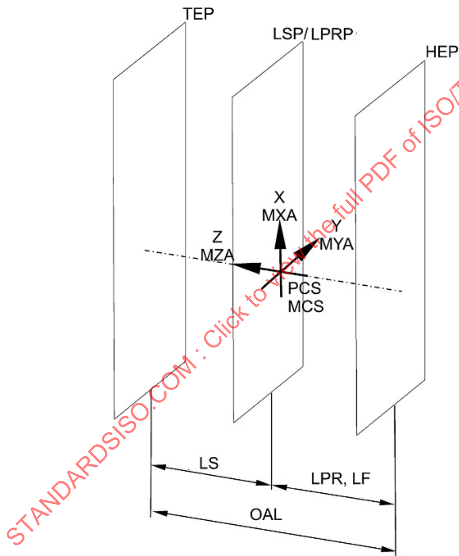
Figure 4 — Planes for design
