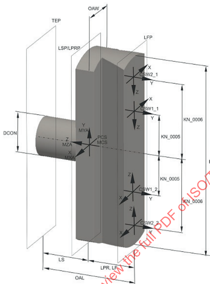
Figure 13 — 3D model of a monoblock extension bridge with adaptor
