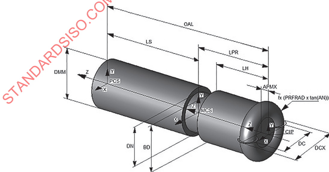
Figure 37 — Basic geometry of rounded end mills
