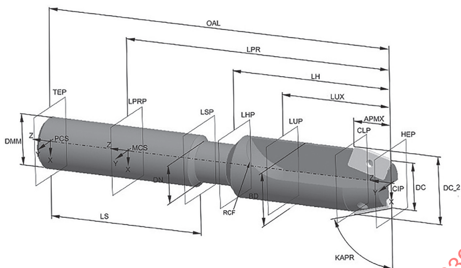
Figure 24 — Assembly of V-groove end mills
