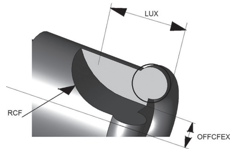
Figure 40 — Chip flute
