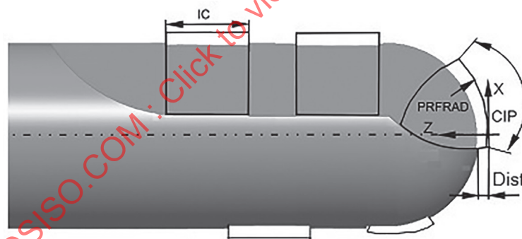
Figure 83 — Chip flute design with inner pocket
