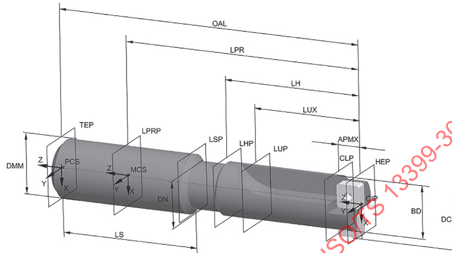
Figure 78 — Assembled spot-facing end mill
