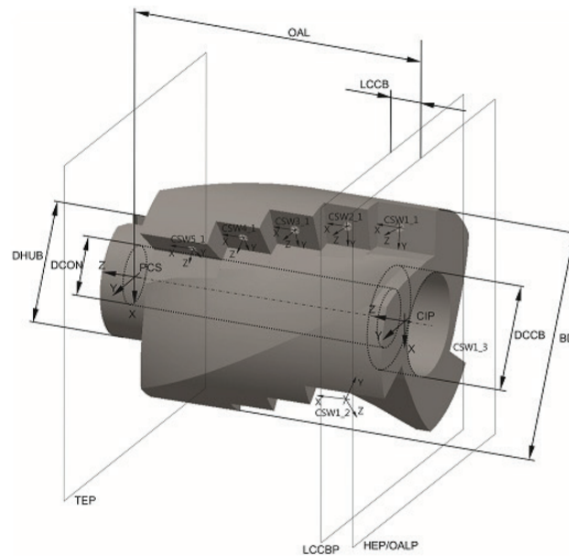
Figure 27 — Arrangement of the pocket seats along the chip flutes
