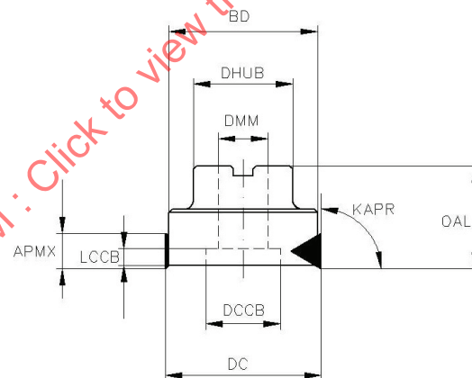
Figure 18 — Determination of properties of shoulder milling cutters
