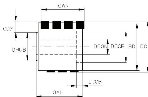
Figure 31 — Determination of properties of shell milling cutters
