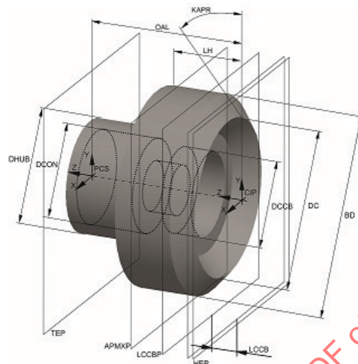
Figure 11 — Basic geometry of face milling cutter
