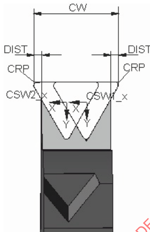
Figure 38 — Determination of CSWs and their positions
