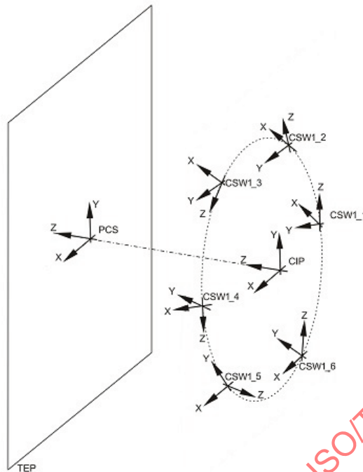
Figure 13 — Location of CSWs of face milling cutters
