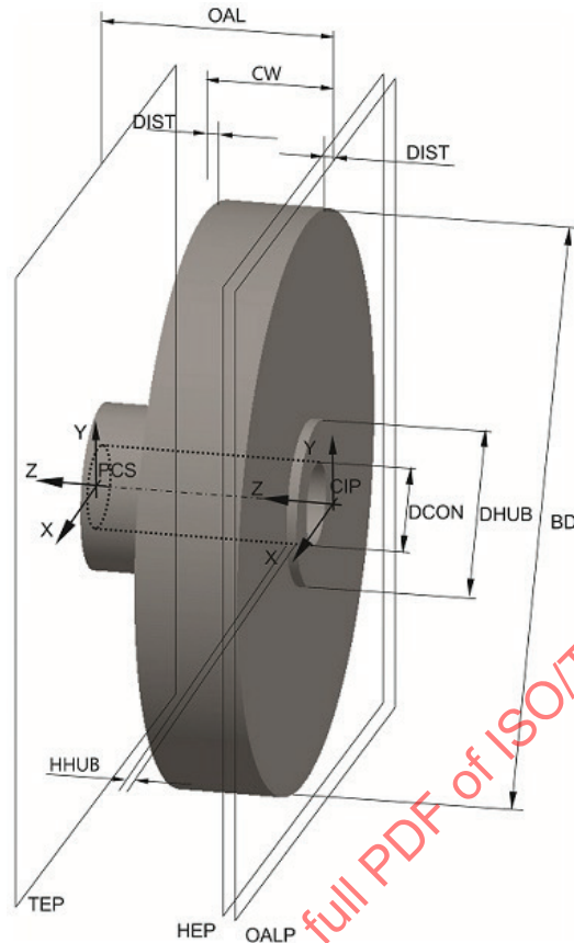
Figure 34 — Basic geometry of a full-side slotting cutter
