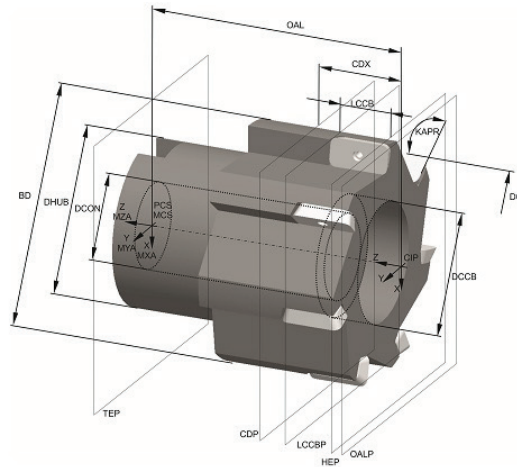
Figure 21 — Shoulder milling cutter, assembly
