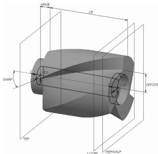
Figure 26 — Design of chip flutes on a plain milling cutter
