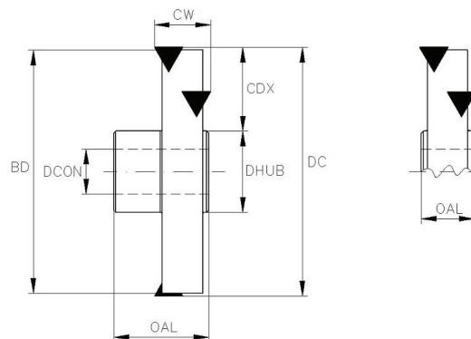
Figure 33 — Determination of properties of full-side slot milling cutters
