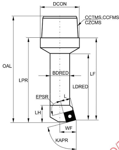
Figure 65 — Determination of properties of system tools for internal turning
