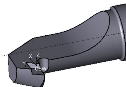
Figure 56 — Boring bar with CSW
