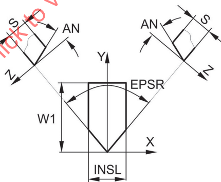
Figure 10 — Tip of type E (angular)
