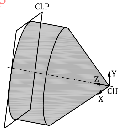
Figure 26 — Revolved body of the cutting part
