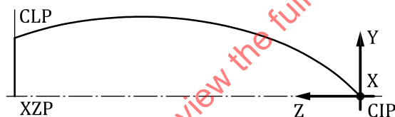
Figure 22 — Sketch of the cutting part
