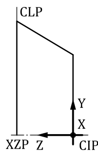
Figure 37 — Sketch of the cutting part
