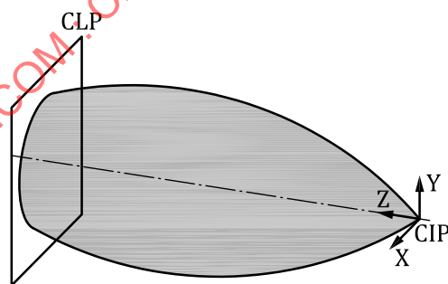
Figure 23 — Revolved body of the cutting part
