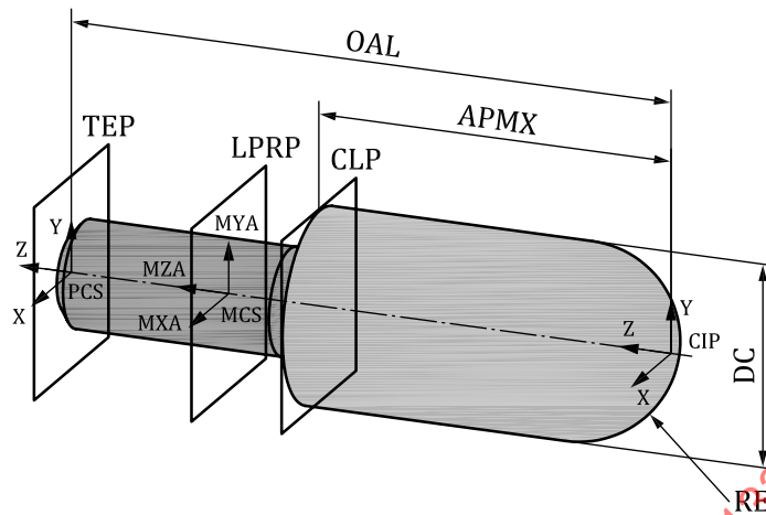
Figure 12 — Completed cylindrical ball-nose burr
