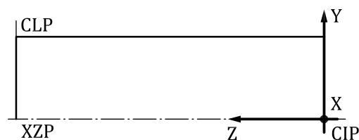
Figure 7 — Sketch of the cutting part
