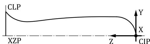
Figure 43 — Sketch of the cutting part
