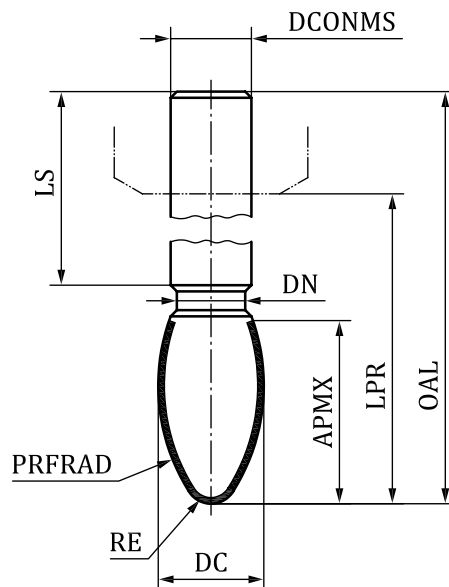
Figure 5 — Determination of general properties for burrs
