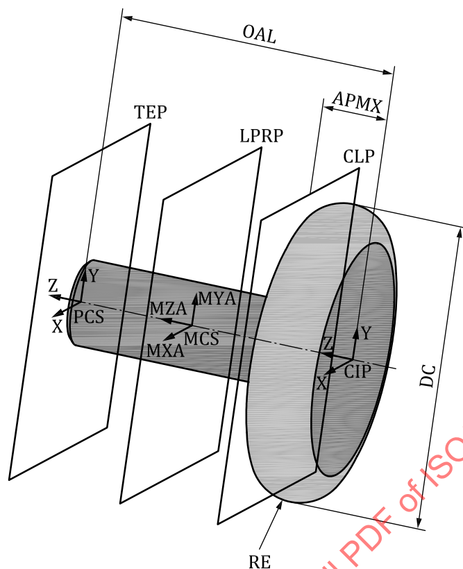
Figure 33 — Completed full rounded disc burr
