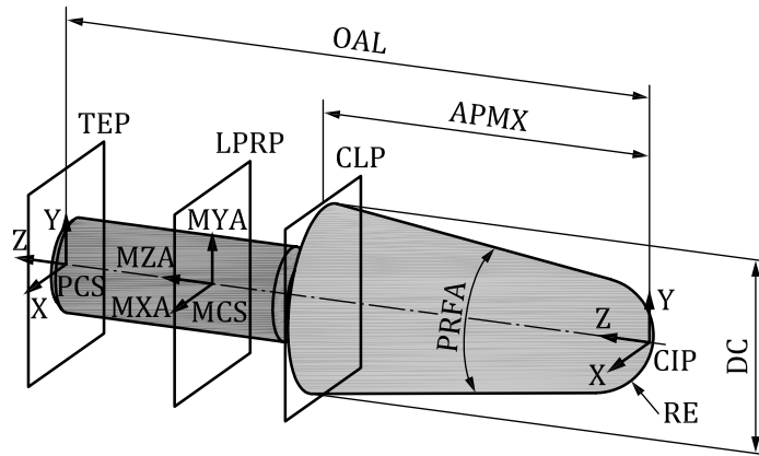
Figure 30 — Completed conical round-(ball-)nose burr
