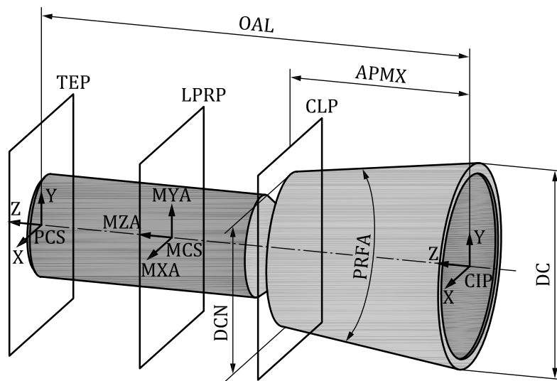
Figure 15 — Completed inverted cone burr
