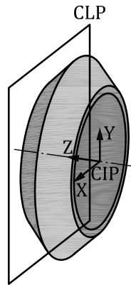
Figure 35 — Revolved body of the cutting part
