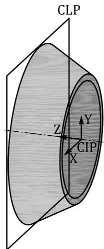
Figure 38 — Revolved body of the cutting part
