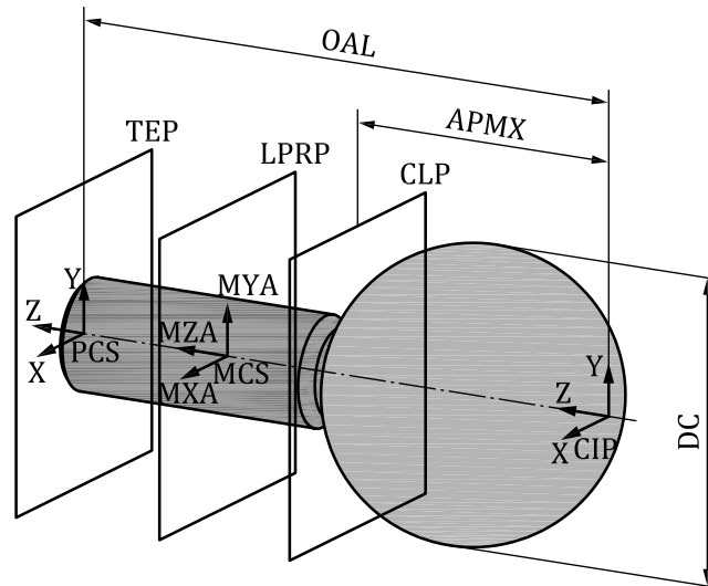
Figure 18 — Completed spherical burr
