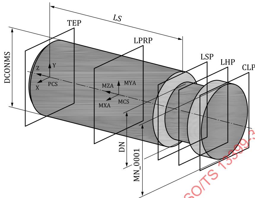
Figure 6 — Non-cutting part including shank
