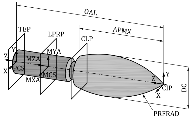
Figure 24 — Arch pointed nose burr
