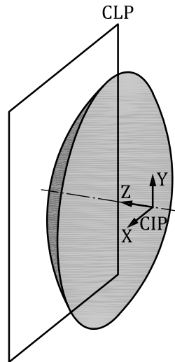
Figure 41 — Revolved body of the cutting part
