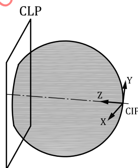
Figure 17 — Revolved body of the cutting part
