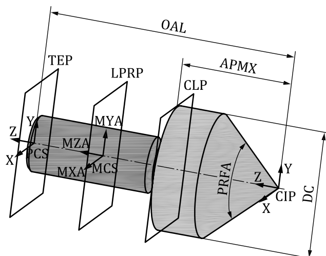
Figure 27 — Completed conical burr
