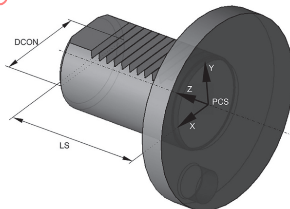
Figure 19 — Connection machine side, complete
