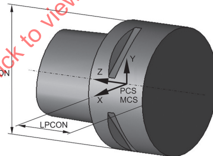
Figure 24 — Connection machine side, complete
