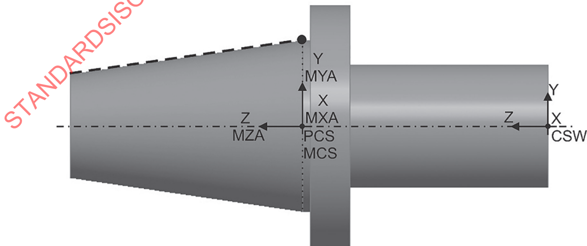
Figure 4 — Example of orientation and location of PCS, MCS and CSW
