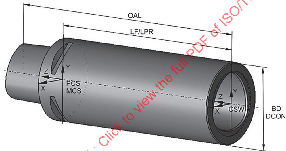
Figure 26 — Extender, complete
