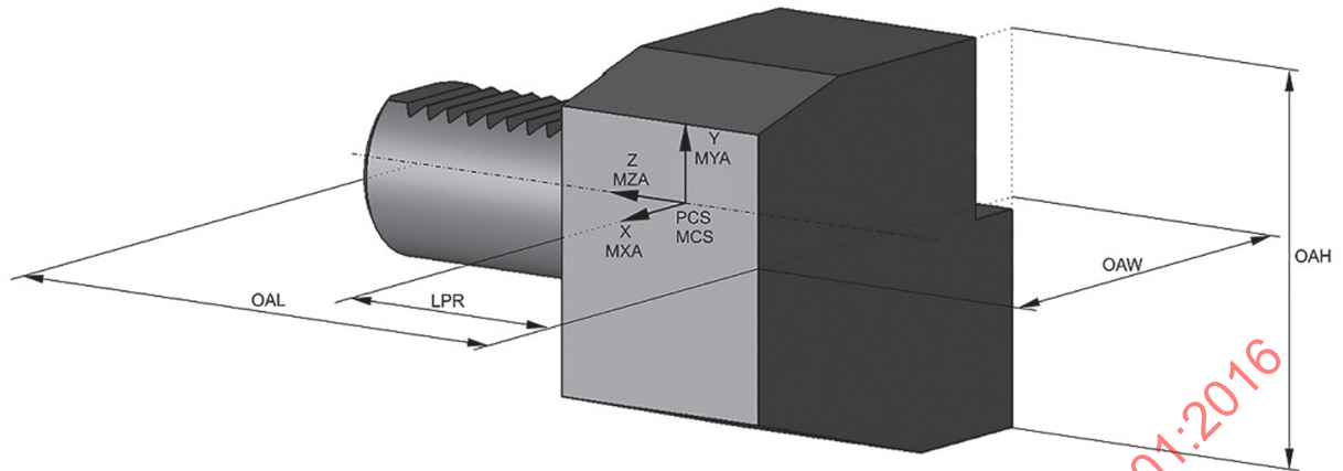
Figure 20 — Basic body
