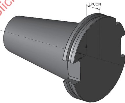
Figure 9 — Revolved body of connection
