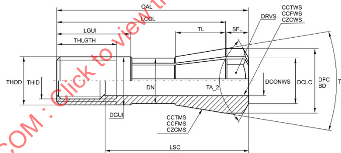
Figure 22 — Determination of properties of draw-in collets with retaining thread and spanner flats
