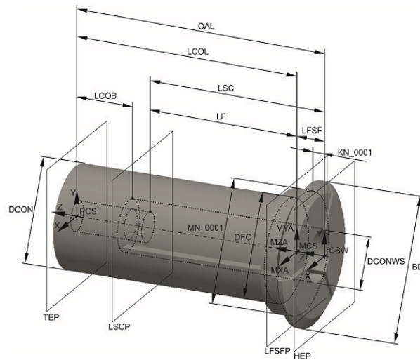
Figure 21 — Completed collet with axial adjustment without drive feature
