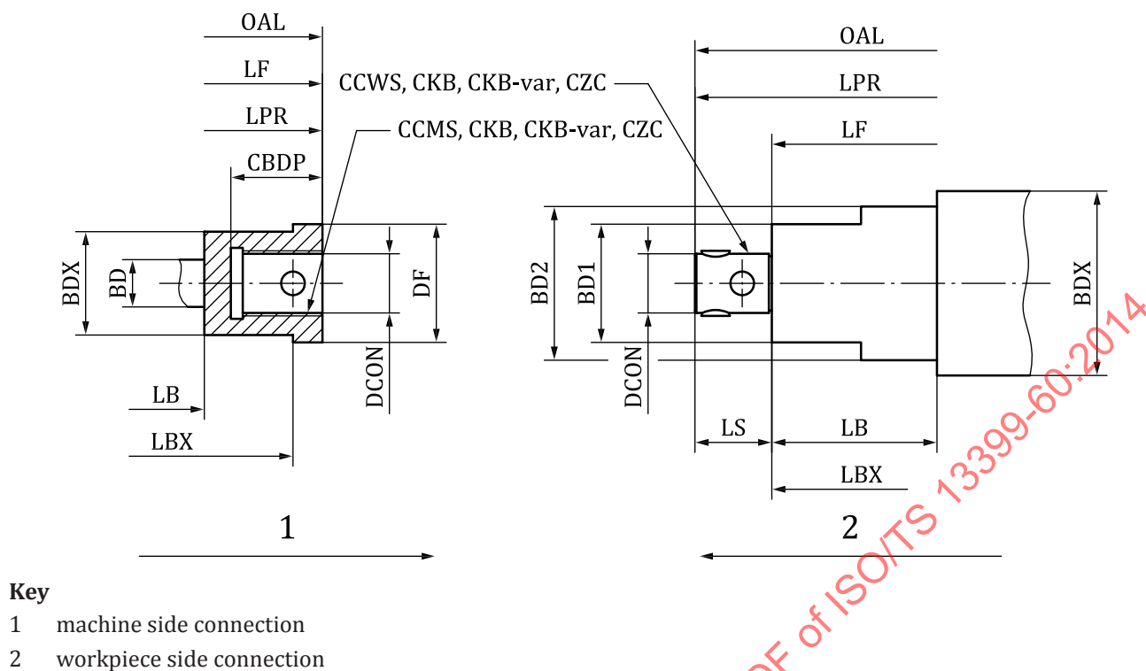
Figure E.20 — Variant 01 of CKB Kaiser bore connection
