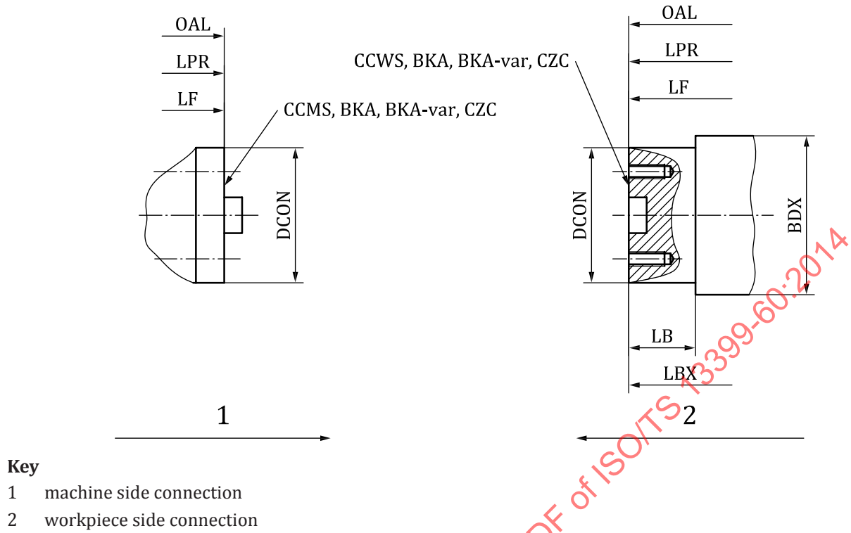
Figure E.5 — BKA boring head connection
