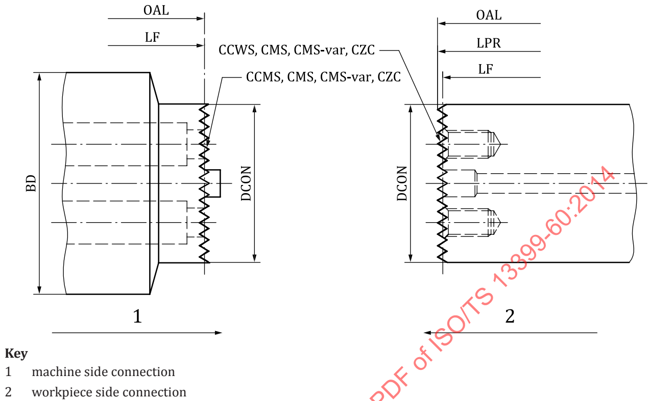
Figure E.22 — CMS Coromant Modular Serrated mounting
