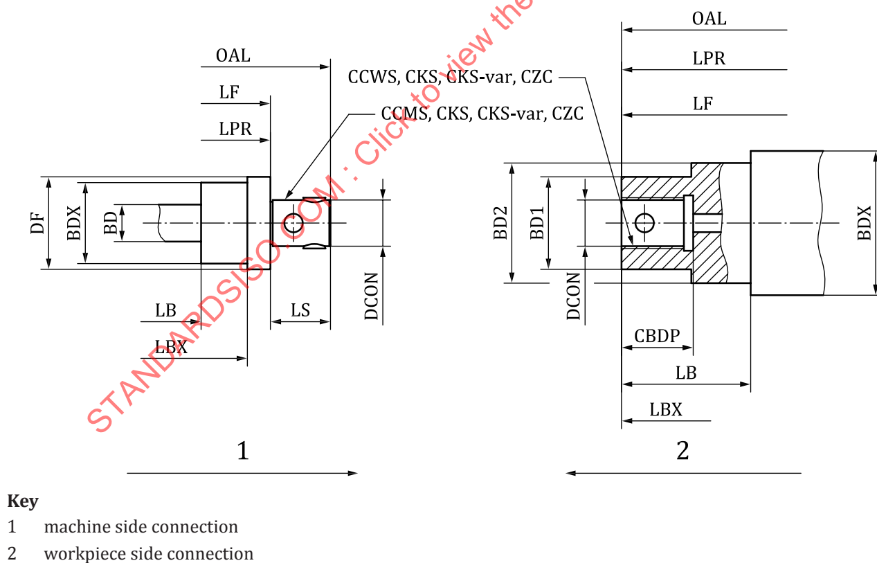
Figure E.21 — CKS Kaiser shank connection
