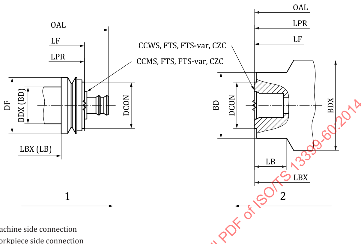
Figure E.28 — FTS flexible tooling system
