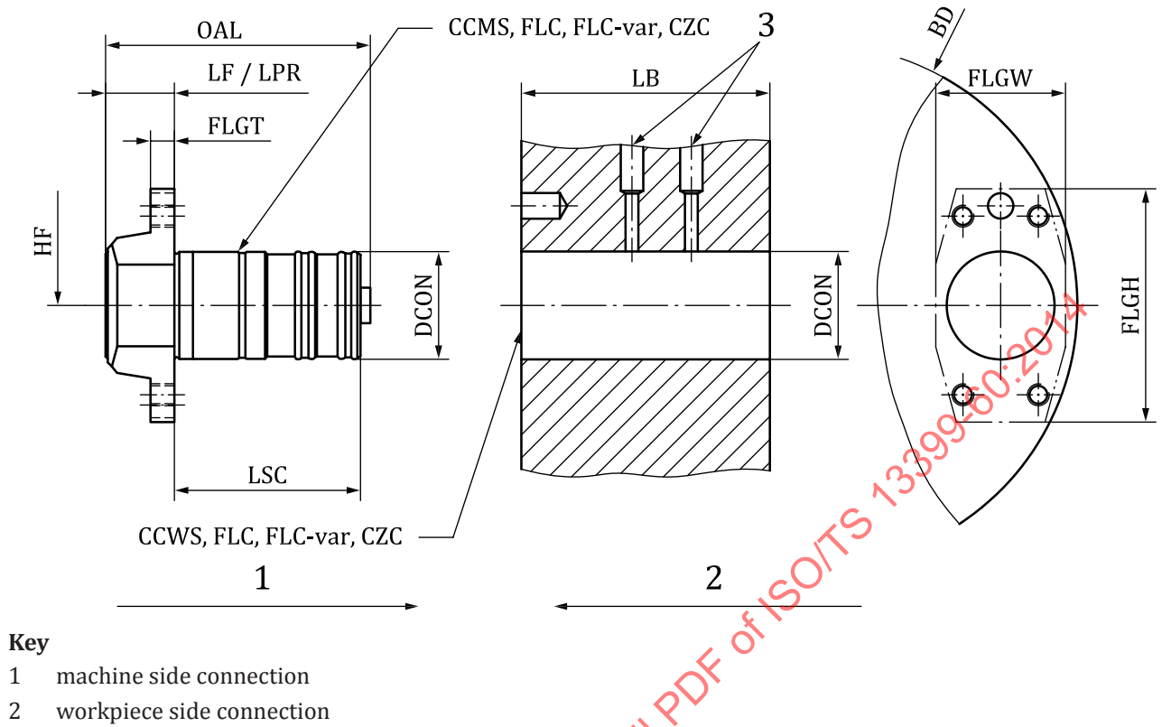
Figure E.26 — FLC flange connection Coromant
