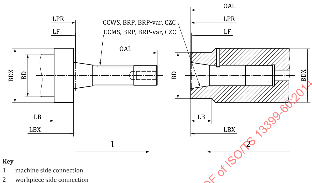
Figure E.7 — BRP Bridgeport connection
