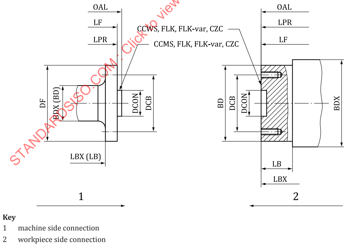
Figure E.27 — FLK flange connector Kennametal
