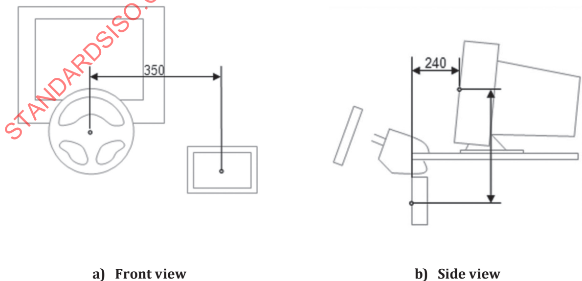
Figure A.1 — Example setup for primary task (LCT example) and secondary task display
