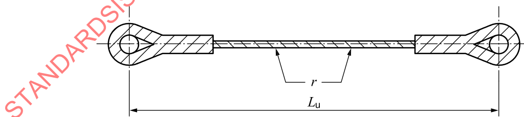
Figure B.1 — Marks, r , on the rope sample
