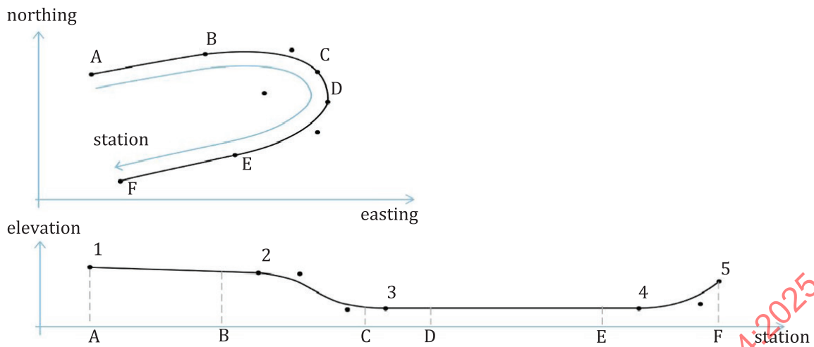
Figure L.5 — Horizontal and vertical alignment
