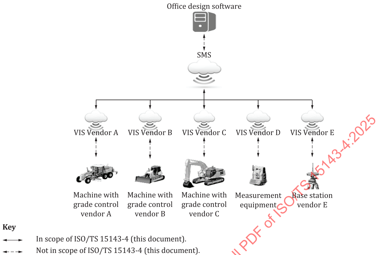
Figure 4.1 — Relationships between VIS and SMS
