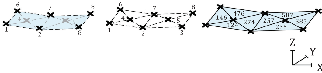
Figure L.2 — Triangulated mesh surface
