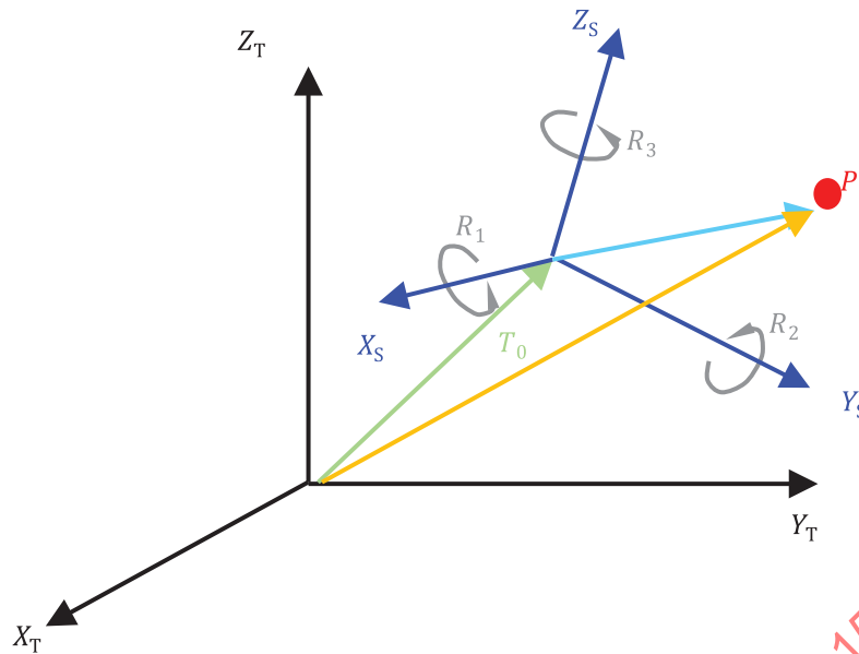
Figure K.1 — Datum sign convention
