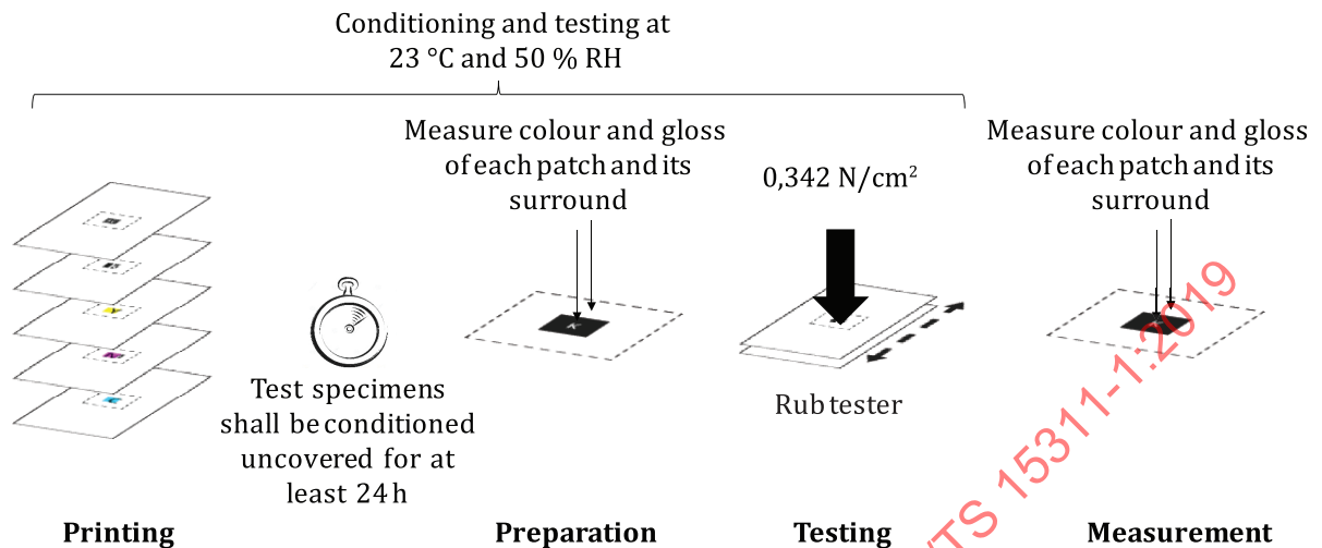
Figure 6 — Abrasion resistance assessment method
