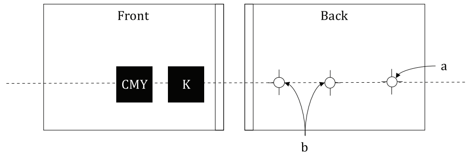
Figure 2 — Test print for measuring print through resistance
