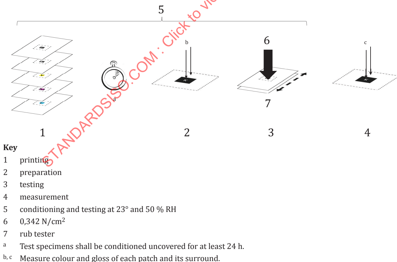
Figure 6 — Abrasion resistance assessment method
