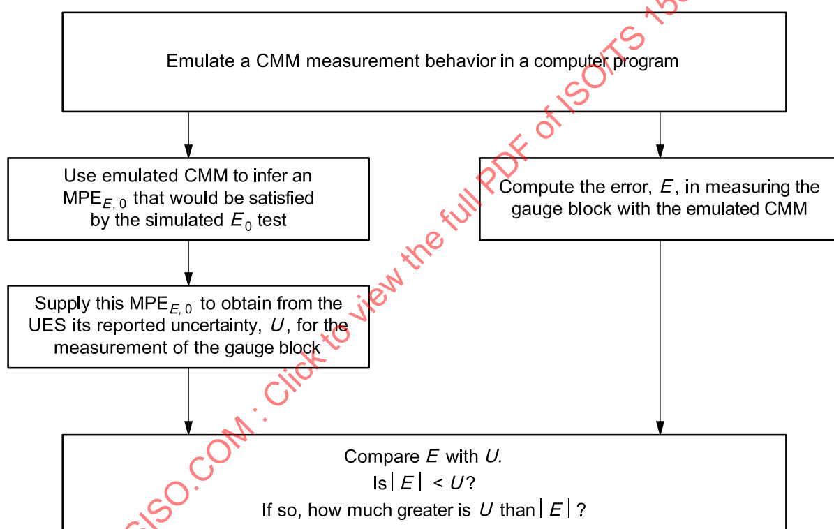
Figure C.2 — A simple CVE flow chart
