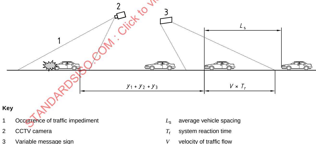
Figure 5 — Image of system reaction time in terms of distance
