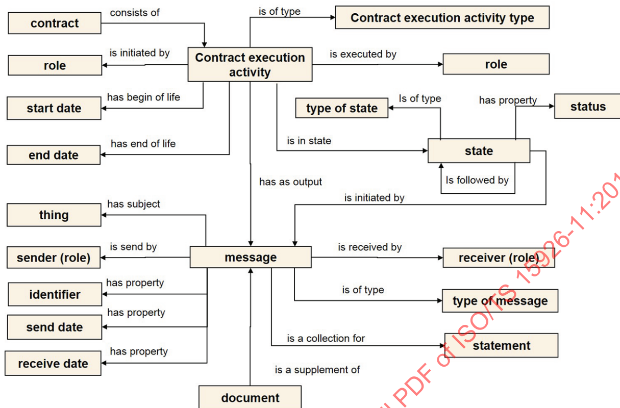
Figure 68 — Information model that represents the communication flow between parties using messages in the context of a specific contract execution activity
