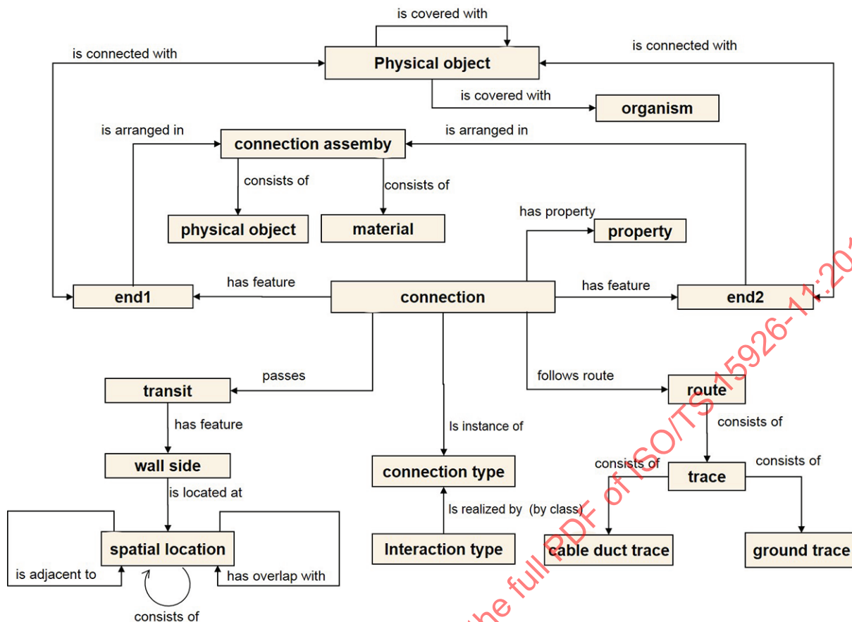
Figure 72 — Information model that represents the connectivity of physical object for example by means of cables and pipes
