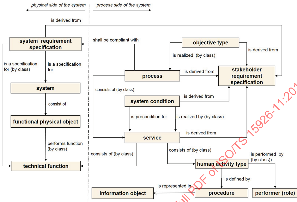
Figure 58 — Information model that represents the process side and the physical side of a system by defining relevant entities and the relationships between these entities concerning the system
