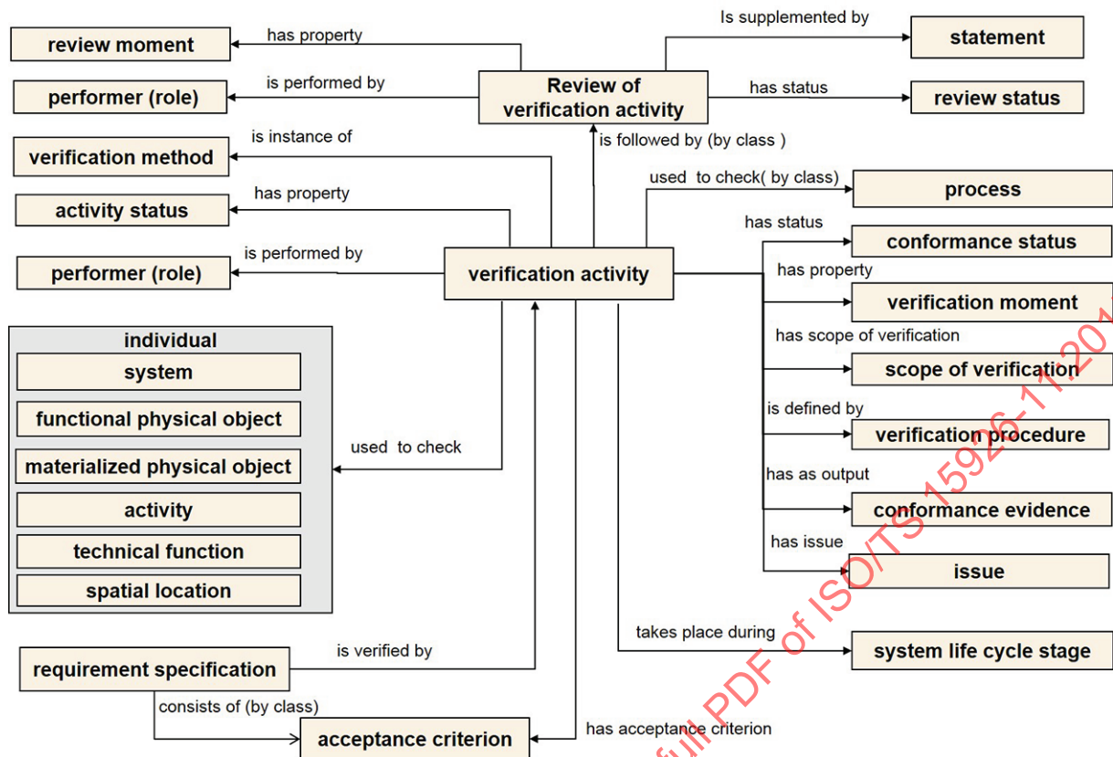
Figure 64 — Information model that represents the verification of a requirement specification by defining relevant entities and the relationships between these entities
