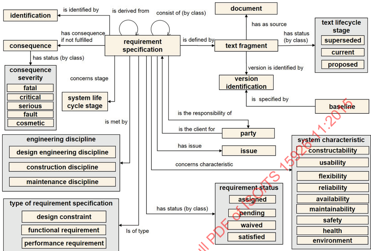
Figure 63 — Information model that represents the requirement analysis of a system by defining relevant entities and the relationships between these entities
