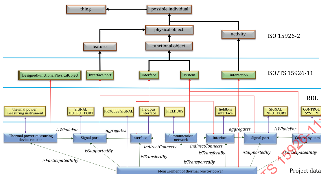
Figure 49 — Example of modelling an interaction being a measurement
