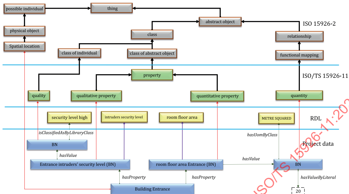
Figure 16 — An example of the modelling of a quantitative and a qualitative property.
