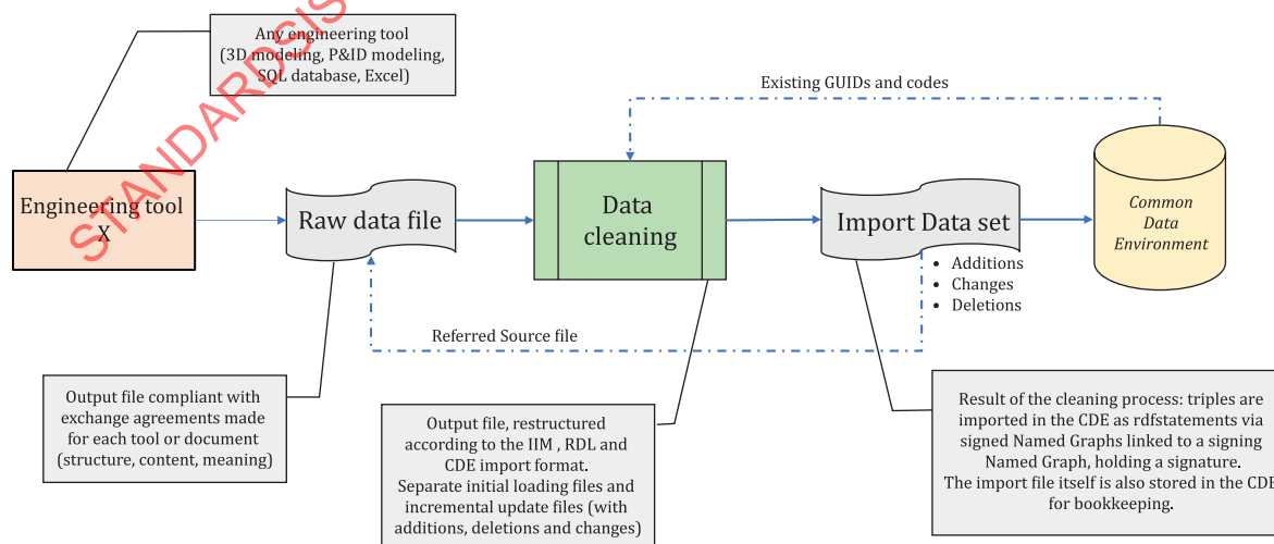
Figure 63 — Typical workflow of processing data files obtained from engineering tools
