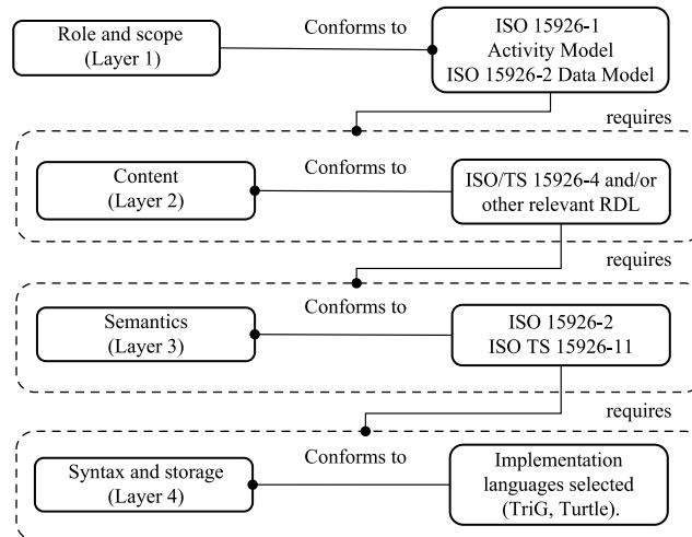
Figure 3 — Layers within the process of data exchange according to this document
