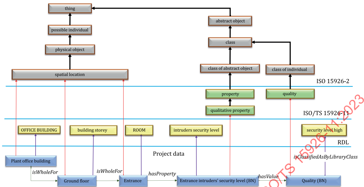
Figure 42 — Modelling pattern of a qualitative property
