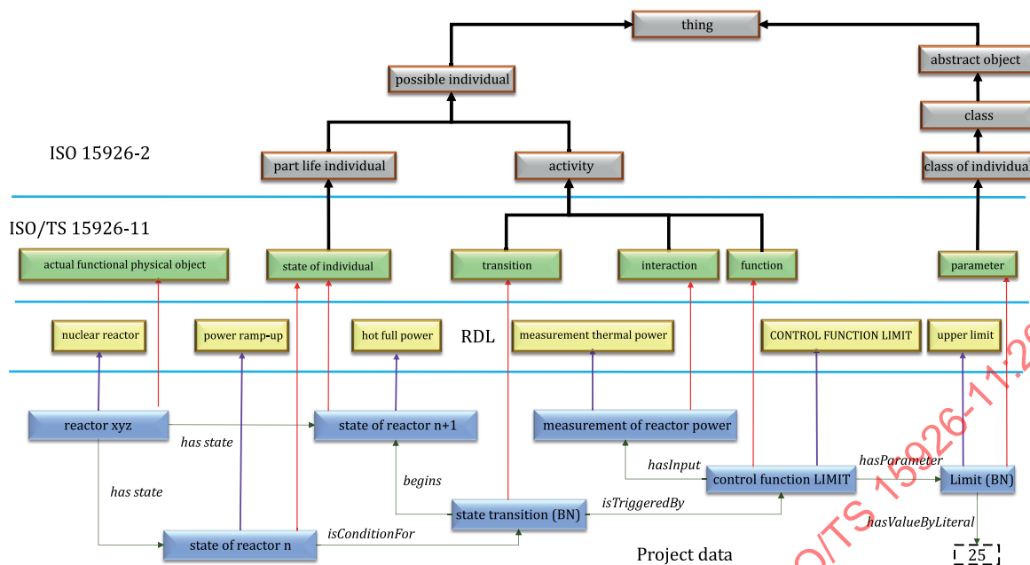
Figure 45 — Modelling of a state of a physical object
