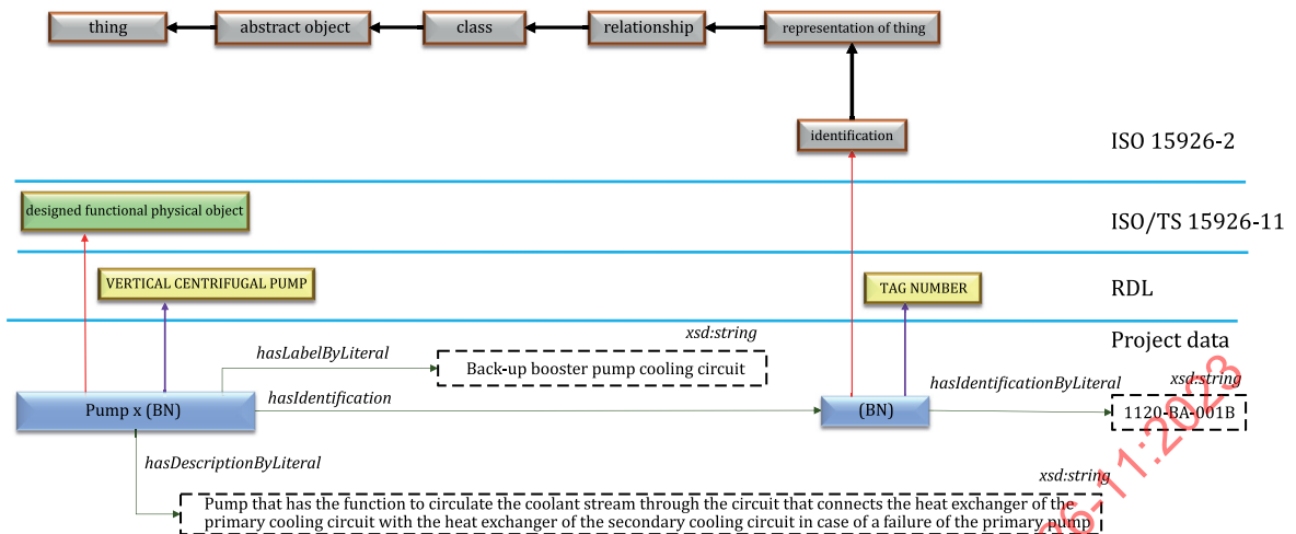
Figure 21 — Examples of relationships of type 'byLiteral' as defined in this document
