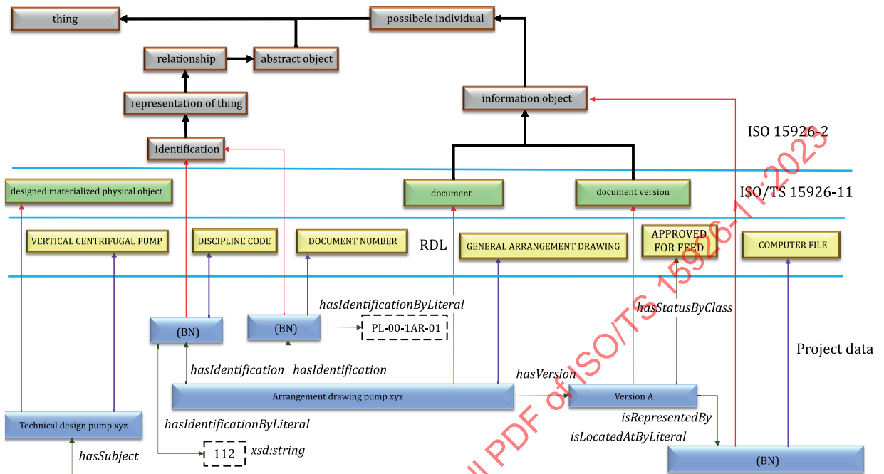
Figure 30 — Example of modelling a document and a corresponding document version
