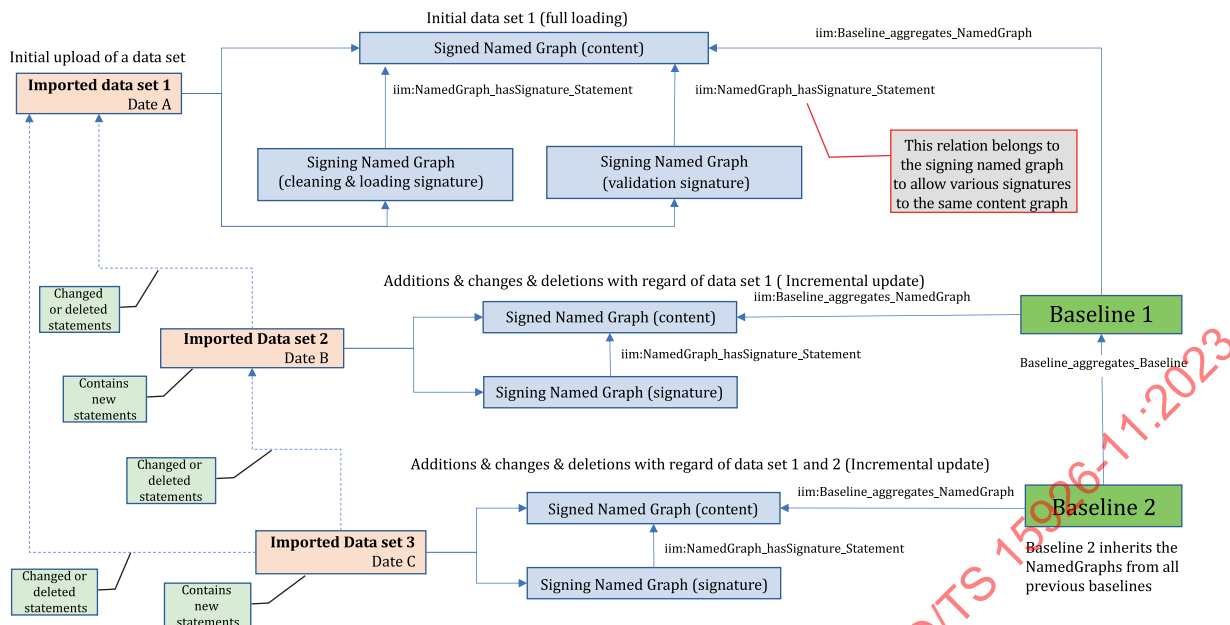
Figure 62 — Typical development of engineering content with respect to additions, deletions and changes, consolidated in baselines
