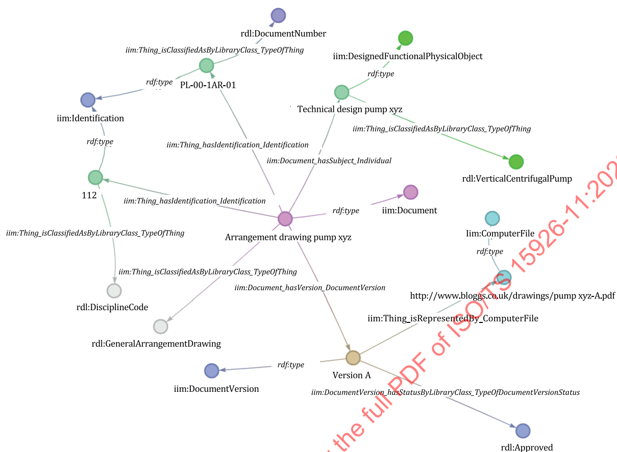
Figure 31 — Implementation of the model of Figure 30 in a graph database application
