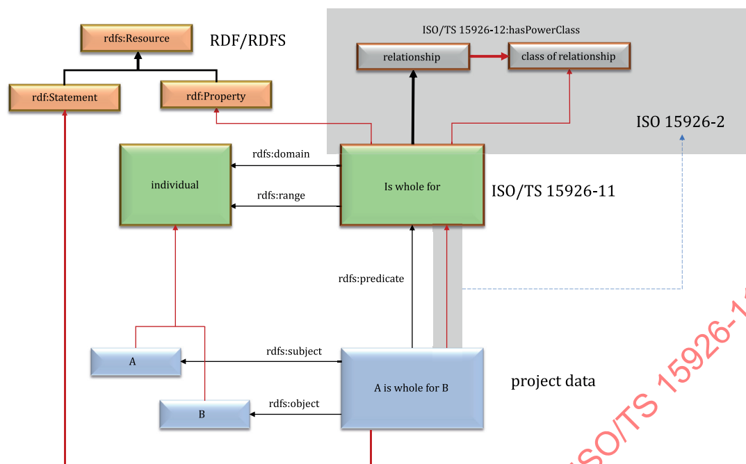
Figure 14 — How relationships of this document connect to ISO 15926-2 and RDFS
