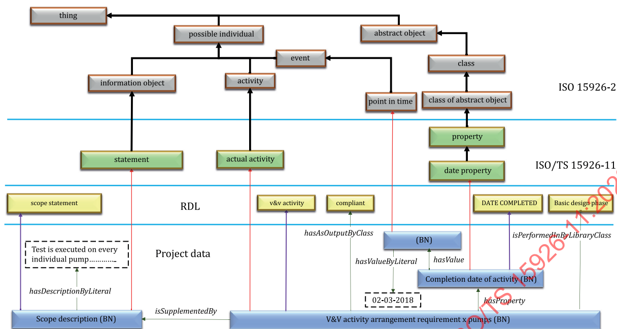
Figure 38 — Example of an actual verification of a requirement
