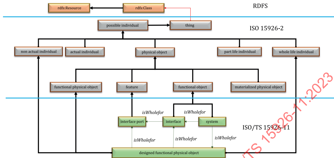
Figure 47 — Entities to model interface of systems in system elements
