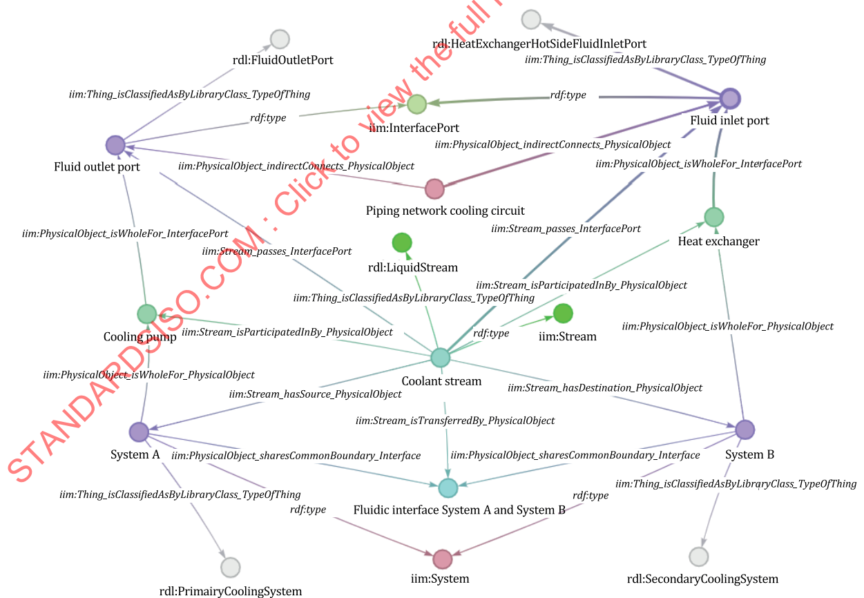
Figure 52 — Implementation of the model of Figure 51 in a graph database application
