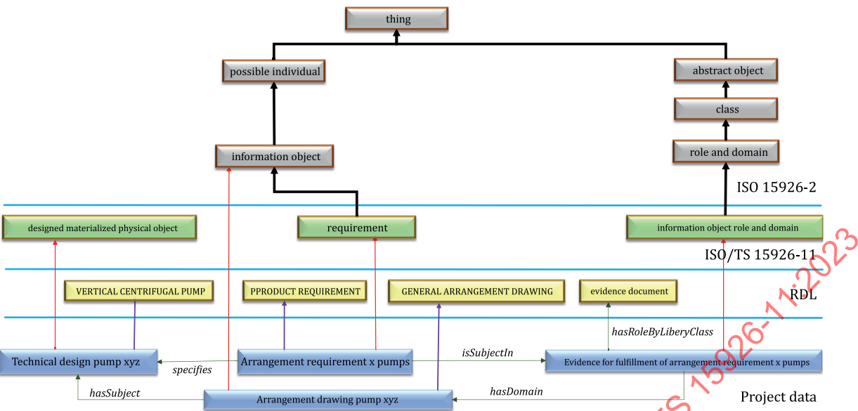
Figure 34 — Example of modelling a requirement and related evidence document
