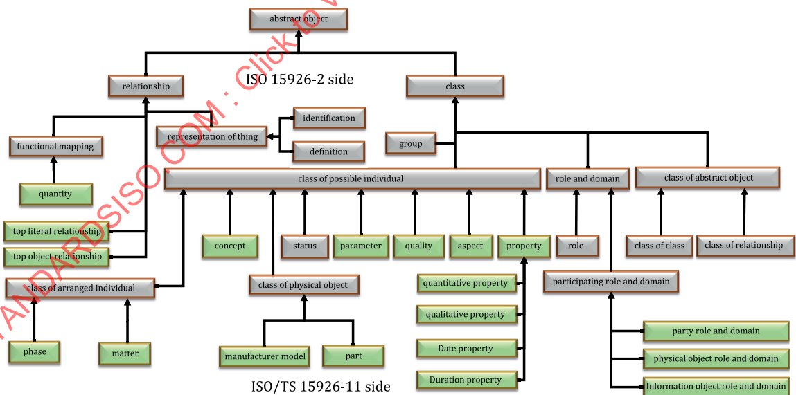
Figure 18 — Expanding ISO 15926-2 abstract object with entities in this document
