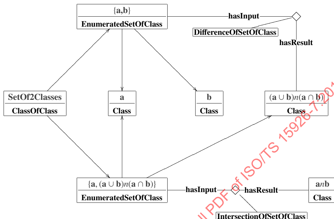
Figure 33 — Example template RelativeComplementOf2Classes
