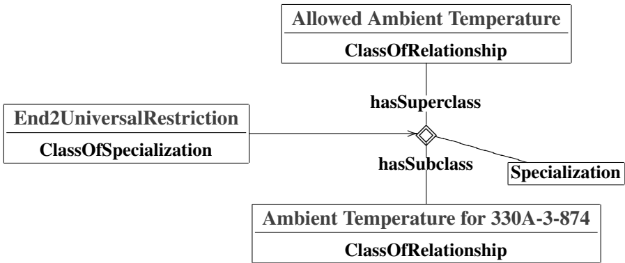
Figure 35 — Example template SpecializationAsEnd2UniversalRestriction
