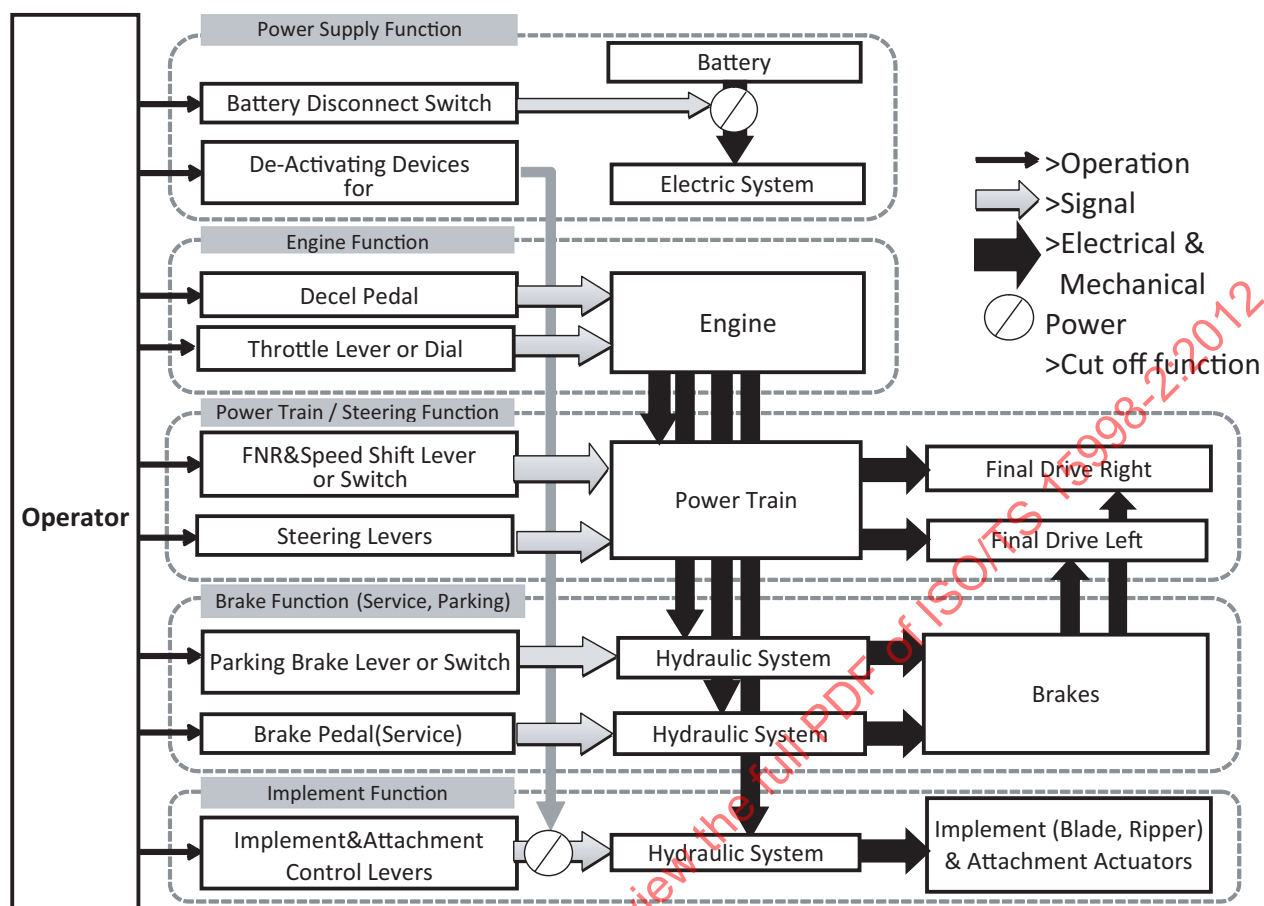
Example of System Block Diagram for Steel-Track Dozer
