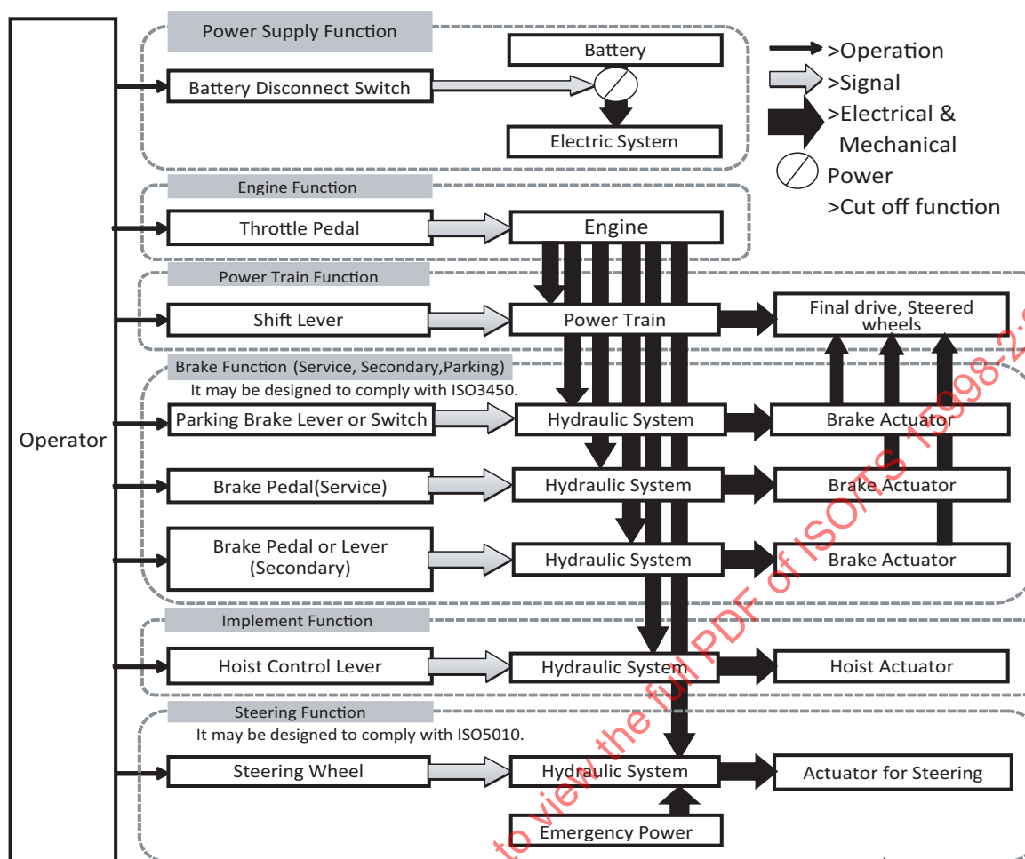
Example of System Block Diagram for Articulated Dump Truck/Rigid Frame Haul Truck
