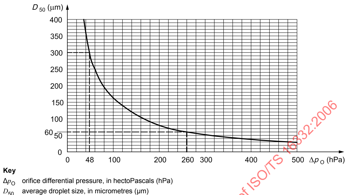
Figure B.4 — Standard curve of average droplet size D_{50} vs orifice differential pressure \Delta p_O
