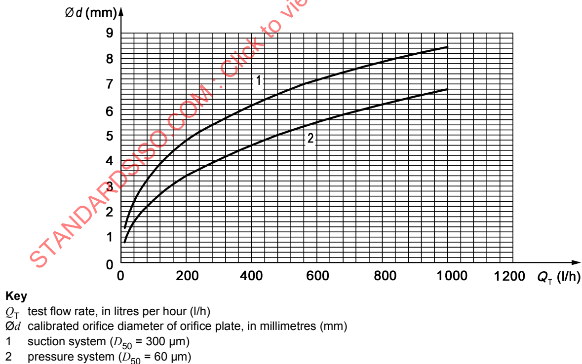
Figure B.5 — Curves relating diameter d of calibrated orifices and fuel test flow rate Q_T for filters of pressure and suction systems
