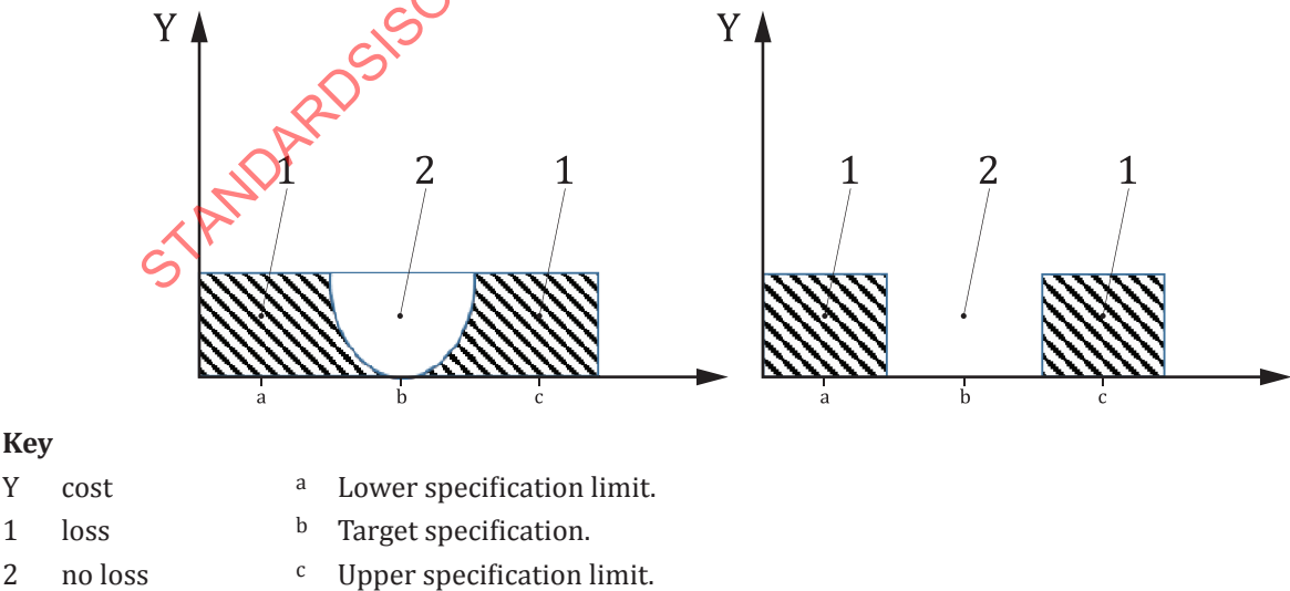
Figure 1 — Taguchi (left) and specification (right) loss function
