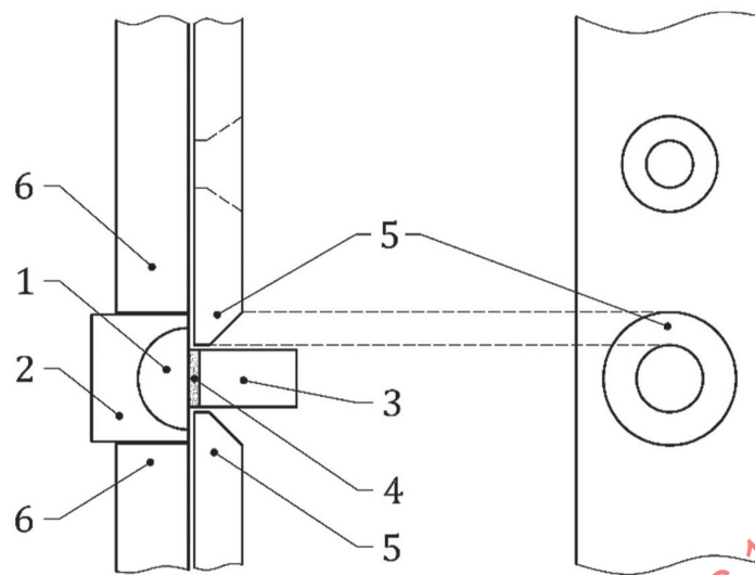
a) Type 1 shear loading jig
