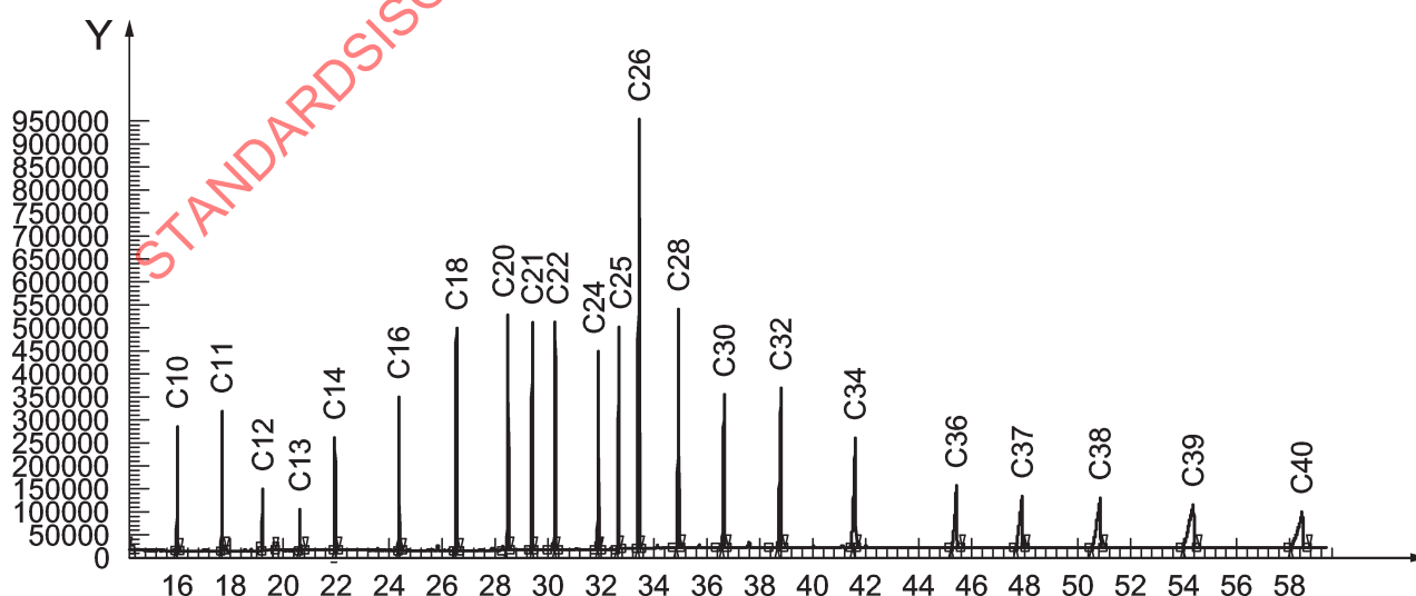
Figure C.2 — Example of a chromatogram of n -alkanes in aliphatic fraction after silicagel cleanup
