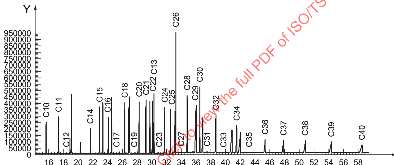
Figure C.1 — Example of a chromatogram of a mixture of n -alkanes/16 EPA PAH before silicagel cleanup
