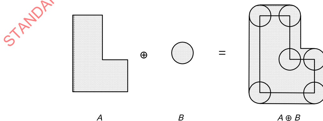
Figure 1 — Minkowski addition of two sets
