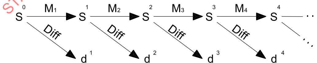
Figure 2 — Schematic representation of the ladder structure of scale space
